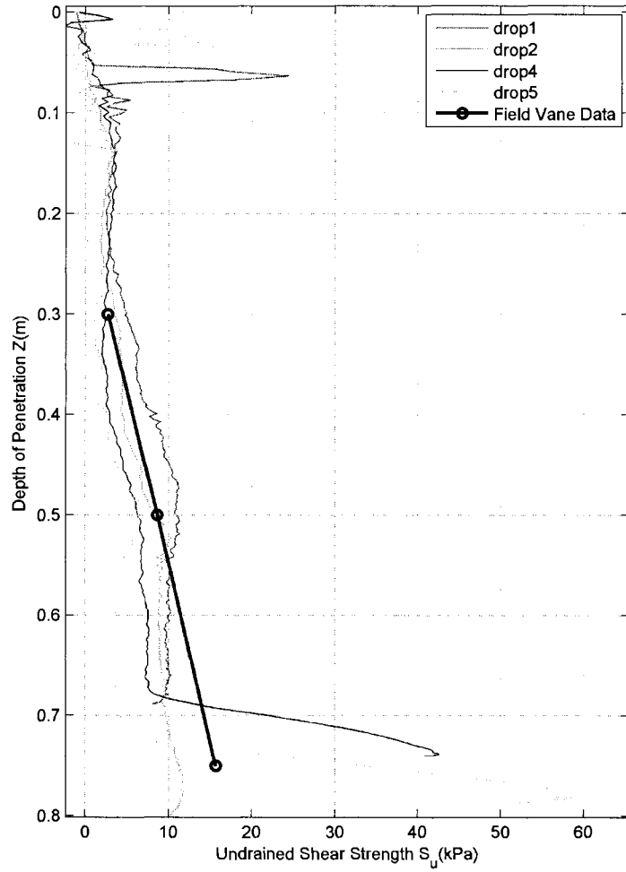
Figure 5-15: Comparison of FFCPT shear strength profiles with data from field vane shear studies at station FP. Values of c_1 = 1.0 and \lambda = 0.15 were used to determine FFCPT data.
