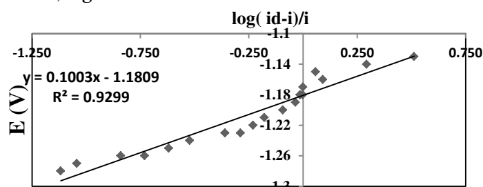
Figure 7: The plot of the applied potential versus \log(i/(id - i)) according to Heyrovsky-Ilkovic equation at 30\mu\text{g.mL}^{-1} of IBU.
