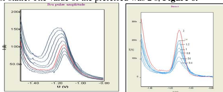
Figure 5: Effect of pulse amplitude on the on the peak current of 25\mu\text{g}\cdot\text{mL}^{-1} IBU in \text{pH} 4 phosphate buffer.
