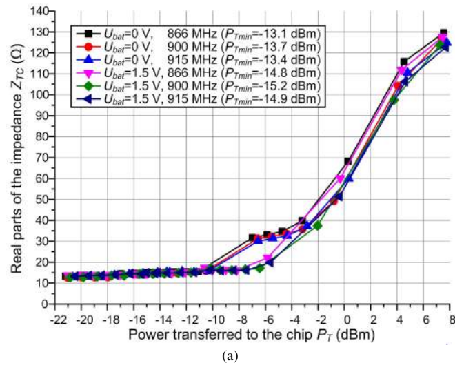
Fig. 11. Measurement results of impedance for passive chip (type 1).
