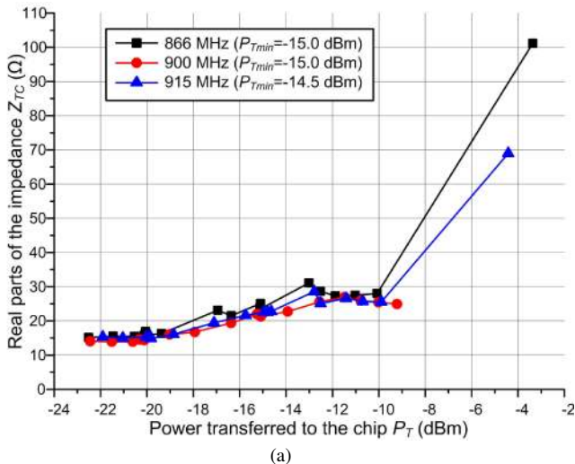
Fig. 12. Measurement results of impedance for passive/semi-passive chip (type 2).
