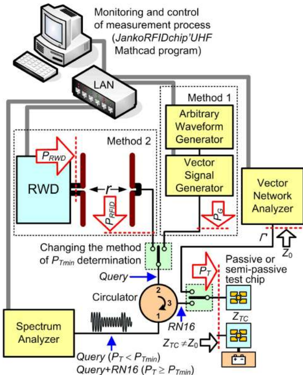
Fig. 5. Block diagram of test stand.
