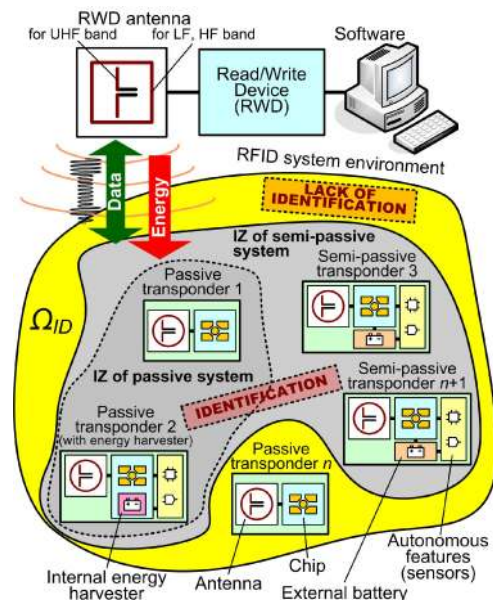
Fig. 1. Generalized block diagram of passive and semi-passive RFID system.
