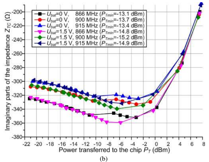
Fig. 12. Measurement results of impedance for passive/semi-passive chip (type 2).
