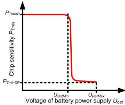
Fig. 3. Generalized curve of sensitivity for passive and semi-passive chip.
