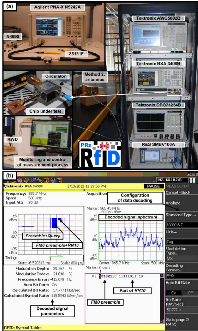
Fig. 8. Equipment of RFID laboratory: a) test stand, b) spectrum analyzer screenshot with decoded data.
