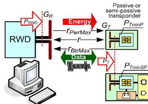
Fig. 2. Passive or semi-passive communication system of RWD – transponder arrangement in UHF band.
