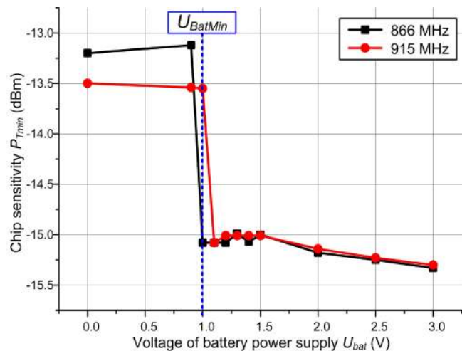
Fig. 10. Measuring results of sensitivity vs. battery voltage for passive/semi-passive chip (type 2).
