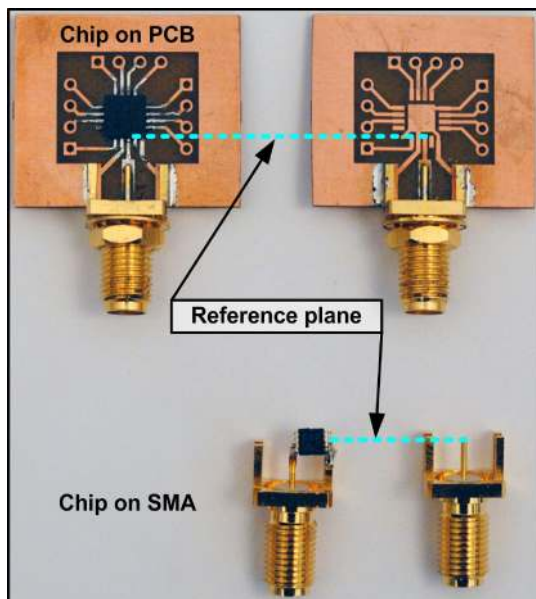
Fig. 9. RFID chips on SMA connector and PCB board.
