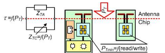
Fig. 4. Electrical equivalent diagram of antenna connected to passive or semi-passive chip.
