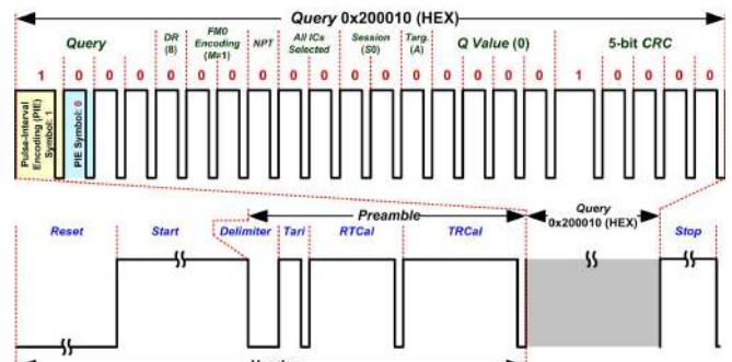
Fig. 7. Frame structure of simulated Query command.
