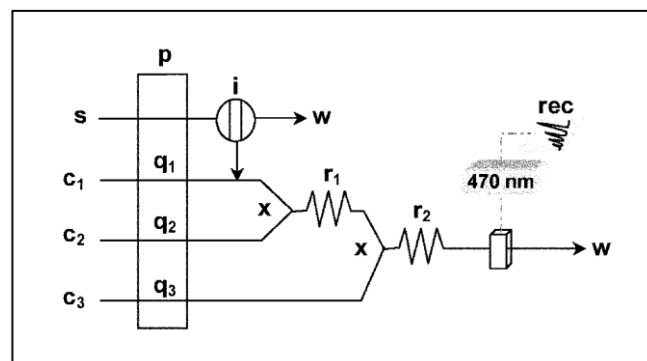
Fig. 1 Flow manifold diagram for determination of polyphenols in wines. s , sample; c _1 , buffer carrier (pH 11); c _2 , HCF solution (9 g L ^{-1} ) carrier, prepared in buffer of pH 11; c _3 , AAP solution (1.7 g L ^{-1} ) carrier, prepared in buffer of pH 11; p , peristaltic pump; q _1 + q _2 + q _3 , overall flow-rate of 1.5 mL min ^{-1} ; i , injection volume (500 \square L); x , confluence points; r _1 and r _2 , reaction coils of length 200 and 10 cm, respectively; w , waste; rec , recorder of spectrophotometric readings at 470 nm
