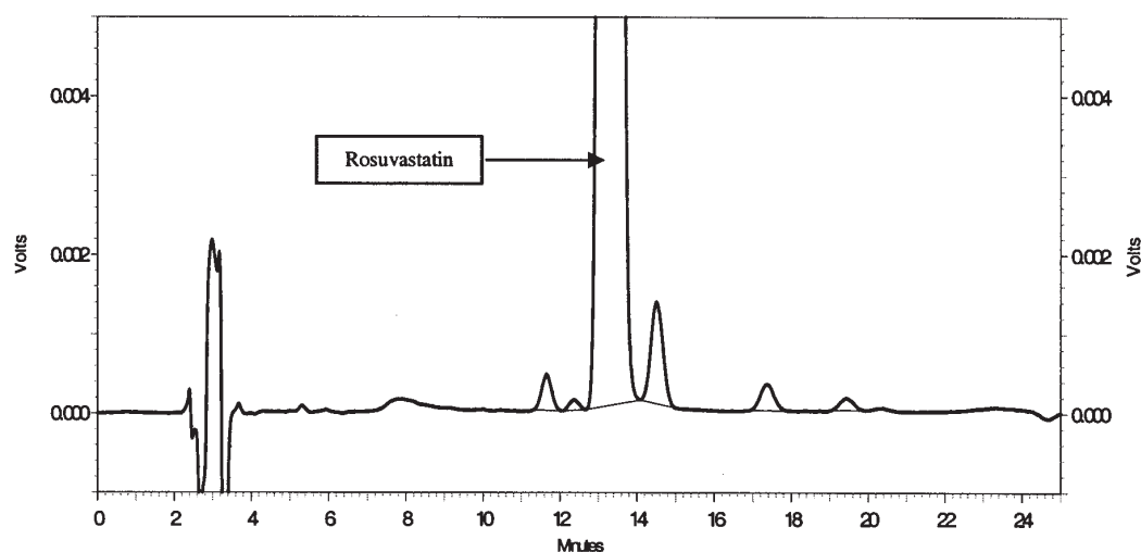
Figure 7. Chromatogram indicating degradation of rosuvastatin Ca in tablet dosage form after exposed for 1 month at 60°C.
