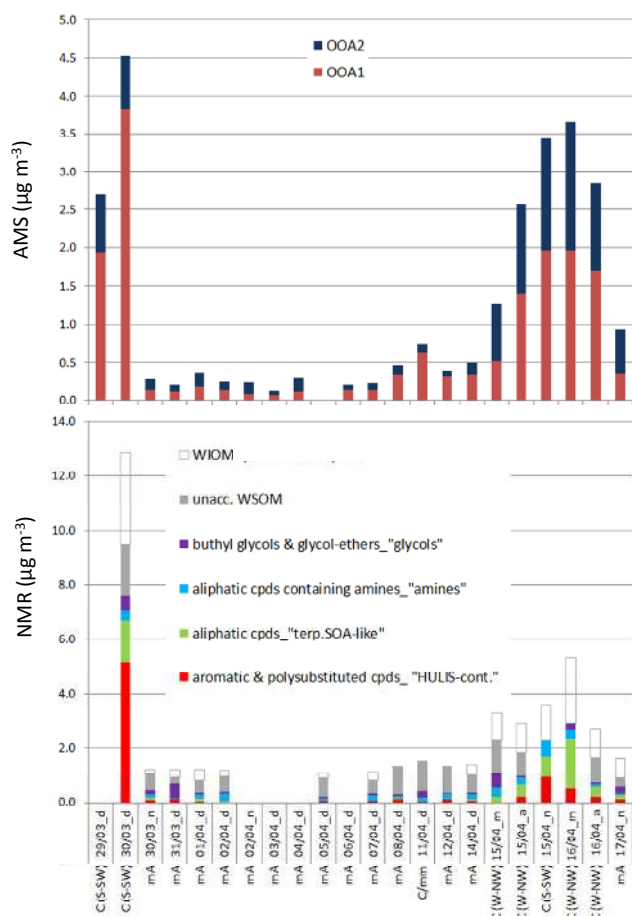
Fig. 11. OM apportionment by factorization of AMS- and NMR-data. Upper panel: Q-AMS-factor contributions averaged upon filter sampling times. Lower panel: unaccounted water-soluble and insoluble OM classes have been included. No data have been reported for NMR samples below detection limits.
