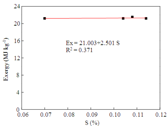
Fig. 5. Relationship between exergy value and S
