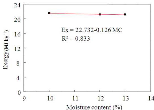
Fig. 3. Relationship between exergy value and moisture
