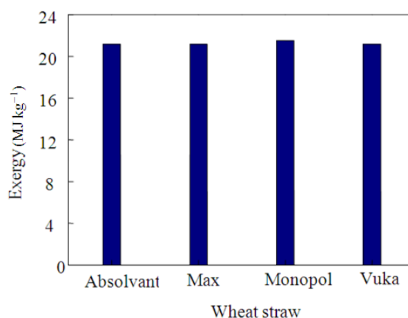
Fig. 1. Exergy values of wheat straws
