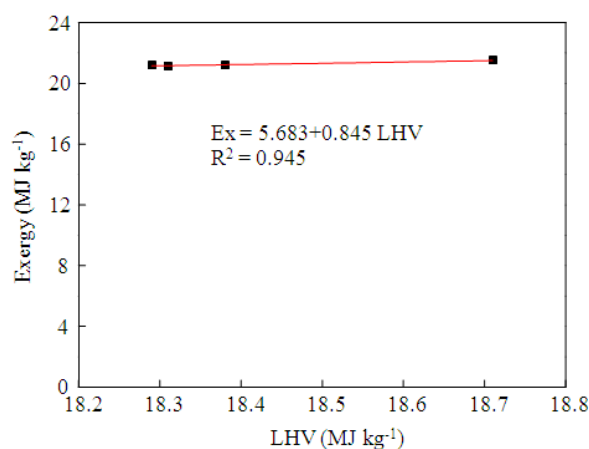
Fig. 2. Relationship between exergy value and LHV
