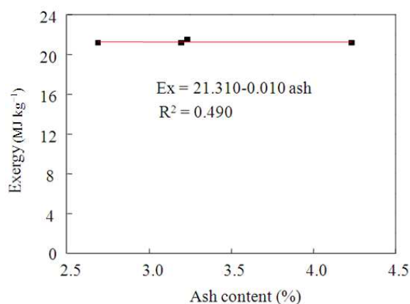
Fig. 4. Relationship between exergy value and ash content
