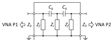
Fig. 2. Equivalent circuit of ring resonator
