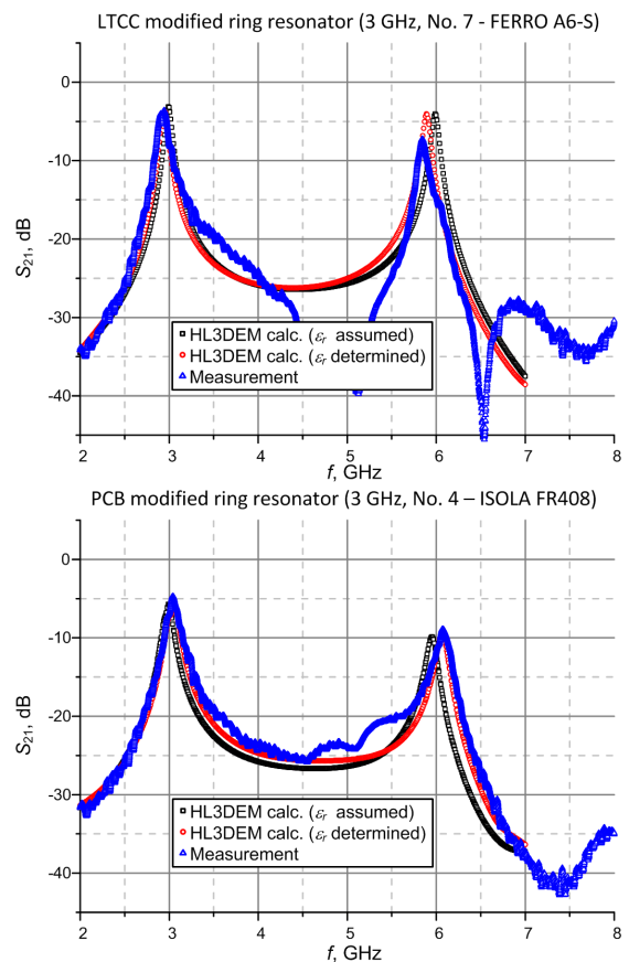
Fig. 7. Examples of results for modified ring resonator and 3 GHz.
