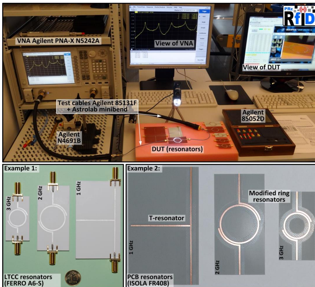
Fig. 4. Test stand in the RFID laboratory.
