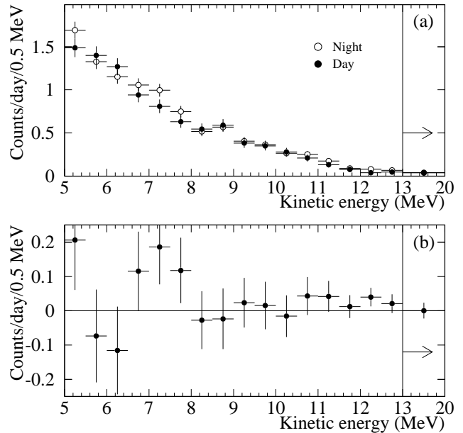
FIG. 45: (a) Energy spectra for day and night. All signals and backgrounds contribute. The final bin extends from 13.0 to 20.0 MeV. Numerical values for each bin are given in Table XXXI in Appendix 14. (b) Difference, night - day , between the spectra. The day rate was 9.23 \pm 0.27 events/day, and the night rate was 9.79 \pm 0.24 events/day.
