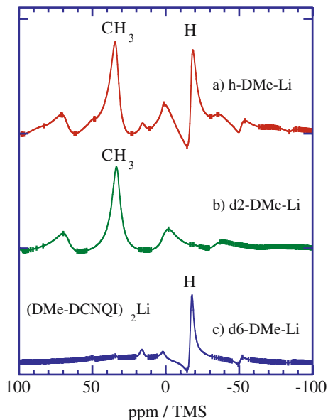
Fig. 2. MAS ^1\text{H} NMR spectra in Li-salt together with the two partially deuterated salts.
