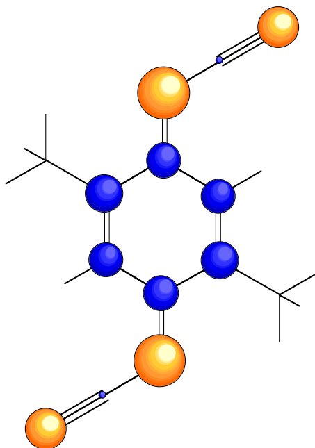
Fig. 3. The obtained charge distribution of the Li-salt. The area represents the relative charge density at each carbon or nitrogen site.
