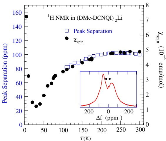
Fig. 1. The temperature dependence of the spin susceptibility measured by EPR-NMR technique and the peak separation of ^1\text{H} NMR splitting in Li-salt.
