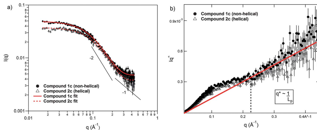
Fig. 4 Small angle neutron scattering (SANS) shows the relatively short persistence length of both polypeptoids. The model fits are shown in (a), demonstrating good fits for the data. In addition, lines with scalings of -1 (rigid rod) and -2 (Gaussian coil) have been added as references. The intensity presented here is absolute intensity in units of \text{cm}^{-1} . The Kratky plot in (b) emphasizes the change in scaling behavior. Incoherent background has been subtracted from the data before the fits.
