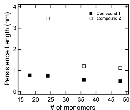
Fig. 5 The persistence lengths of polypeptoids ranging in length from 18 to 48 monomers (Compound 1 series and Compound 2 series) as determined from the wormlike chain model are plotted versus the number of monomers. The shorter chains have significantly higher persistence lengths, indicating that the molecules are too short to be treated using this method.
