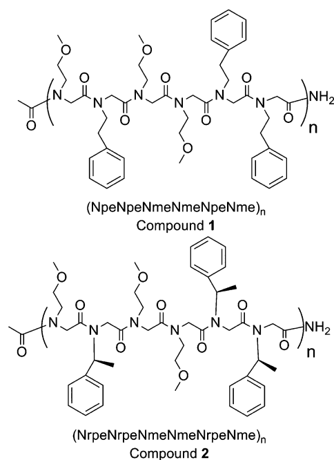
Fig. 1 1 contains achiral aromatic side chains, while 2 , a helix-forming polypeptoid, contains alpha-chiral side chains. The value of n ranges from 3 to 8 for chains of varying lengths.
