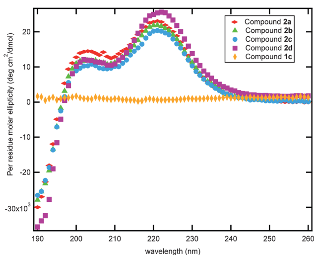
Fig. 2 CD spectra for different chain lengths of a helical polypeptoid as well as a non-helical polypeptoid.
