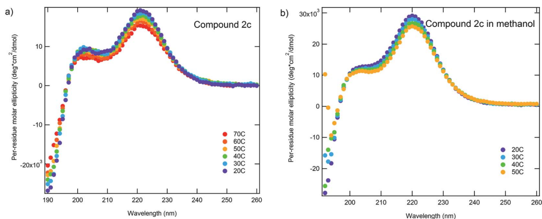
Fig. 3 Heating (a) and solvent (b) do not significantly affect the CD spectra of 2c .
