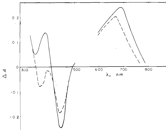
Figure 1. Transient change in absorption observed 8 \mu s after flashing an aqueous solution of lumiflavin; Oxygen-free. ----- pH = 2 lumiflavin ( 10^{-5} M); ——— pH = 7 lumiflavin ( 10^{-5} M); ..... pH = 13 lumiflavin ( 2 \times 10^{-5} M).
