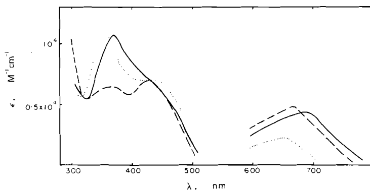
Figure 2. Triplet-triplet absorption spectra (see text) of lumiflavin in aqueous solution 8 \mu s after flashing: ---- pH = 2 acid triplet form ( {}^3\text{LfH}_2^+ ); ——— pH = 7 neutral triplet form ( {}^3\text{LfH} ); ..... pH = 13 basic triplet form ( {}^3\text{Lf}^- ); oxygen-free.
