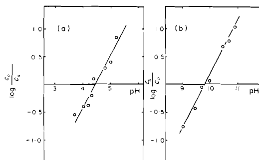
Figure 3. (a) Log plot of the concentration ratio C_n/C_a of the neutral ( {}^3\text{LfH} ) to the acid ( {}^3\text{LfH}_2^+ ) lumiflavin triplet form vs pH. (b) Log plot of the concentration ratio C_b/C_n of the basic ( {}^3\text{Lf}^- ) to the neutral ( {}^3\text{LfH} ) lumiflavin triplet form vs pH. For determination of the concentration ratio, see text.
