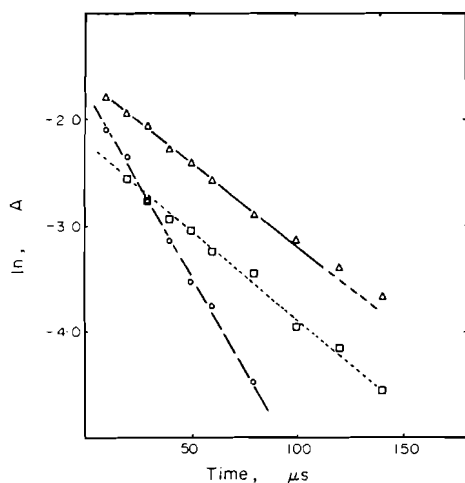
Figure 4. Logarithmic plot of decay of absorbance after flashing 5 \times 10^{-6} M lumiflavin in aqueous solution at different pH values: ---- pH = 2, \lambda_{\text{obs}} = 670 \text{ nm} ; ——— pH = 7, \lambda_{\text{obs}} = 690 \text{ nm} ; . . . . pH = 13, \lambda_{\text{obs}} = 650 \text{ nm} .
