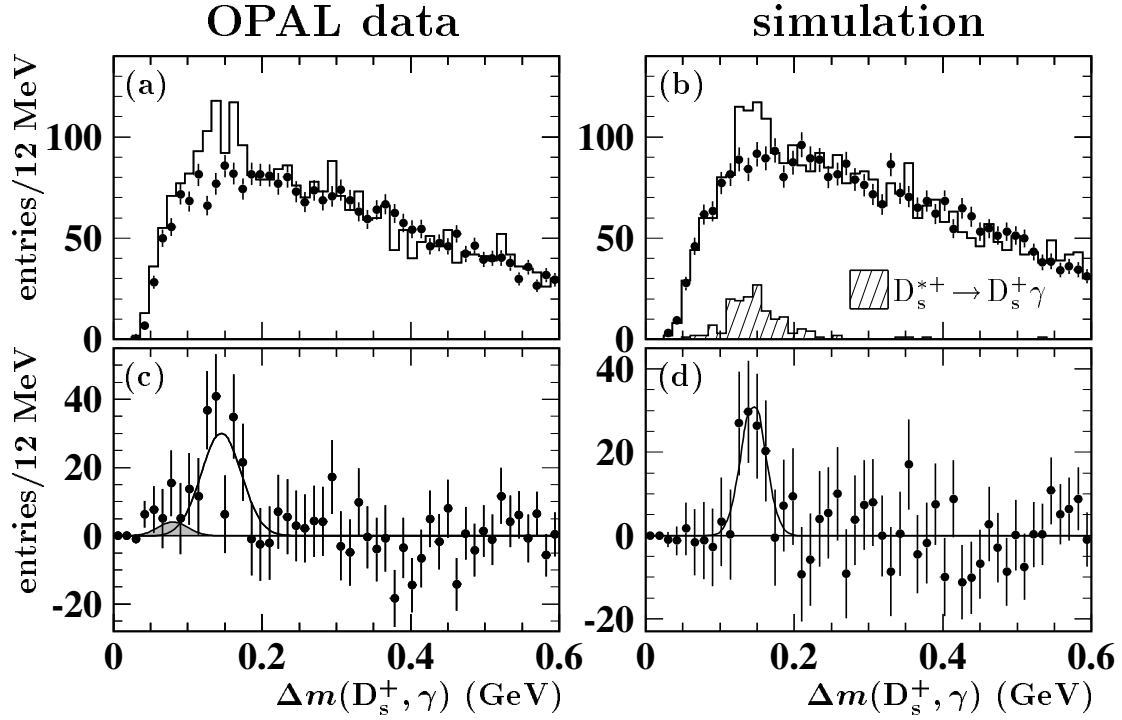
Figure 4: The mass difference distribution for the decay D_s^{*+} \rightarrow D_s^+ \gamma . As before, in (a) and (b), the solid histogram corresponds to the signal sample, and points with error bars to the background sample. The signal contribution in the simulation is indicated by the hatched histogram.
