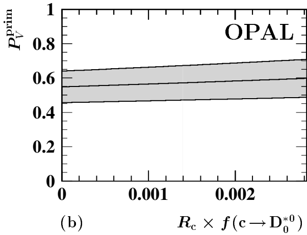
Figure 5: The dependence of P_V^{\text{prim}} on the two unmeasured multiplicities R_c \times f(c \rightarrow D_0^{*0}) and R_c \times f(c \rightarrow D_1^0) is shown in figure (a). Each of these quantities is varied between 0 and twice the value as expected from a spin counting picture. Plots (b) and (c) show the dependence on each one of these multiplicities when the other is fixed at the spin counting expectation. The error contours correspond to one standard deviation. They include the experimental error on the relative production of D_1^0 and D_2^{*0} mesons as measured in [10].
