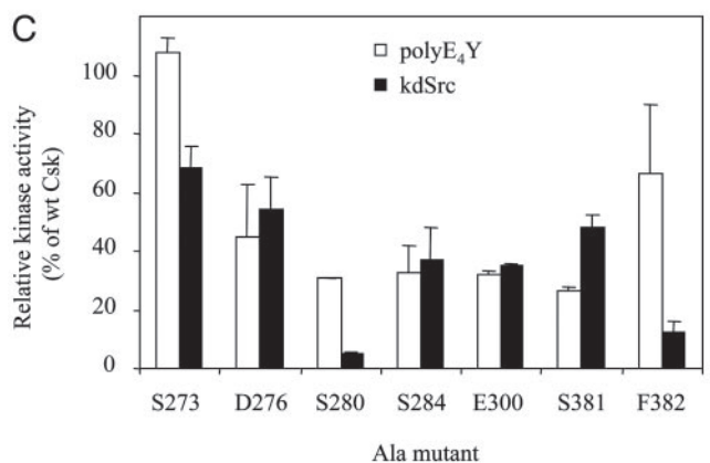
Fig. 2. Ala scanning mutagenesis to identify the substrate-docking site on Csk. (A) Ala scanning of polar or charged residues that are uniquely conserved in the Csk family. The activity of the Ala mutants toward an artificial and a physiological substrate are determined. (B) Structure of the Csk peptide-binding lobe. Residues that are potentially part of the substrate-docking site, the catalytic loop, and the activation loop are indicated. (C) Ala scanning of residues in or near the identified substrate-docking site.
