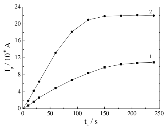
Figure 3. Effect of preconcentration time on the peak current. Open-circuit preconcentration in (1) 5.0 \times 10^{-8} mol/L Sb (III); (2) 1.0 \times 10^{-7} mol/L Sb (III). Other conditions as in Figure 2, curve 3.
