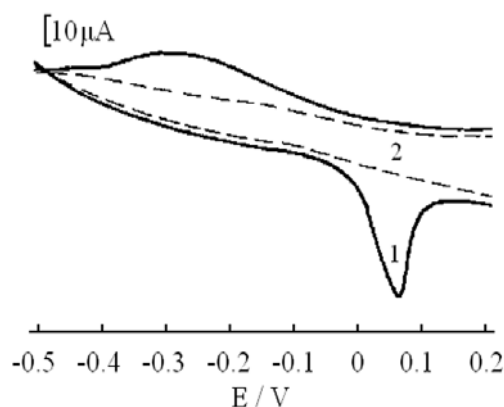
Figure 4. Cyclic voltammograms of the CPE pre-concentration in 0.10 mol/L HCl solution containing 1.0 \times 10^{-6} mol/L Sb (III) and 3.0 \times 10^{-5} mol/L PGR. (1) the first scan; (2) the repetitive scan. Scan rate: 50 mV/s, other conditions as in Figure 2, curve 3.
