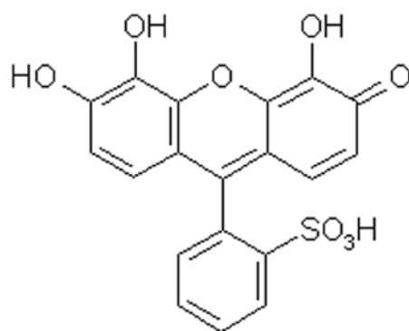
Figure 1. The structure of pyrogallol red (PGR).
