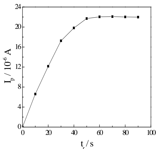
Figure 7. Effect of reduction time on the peak current. Other conditions as in Figure 2, curve 3.
