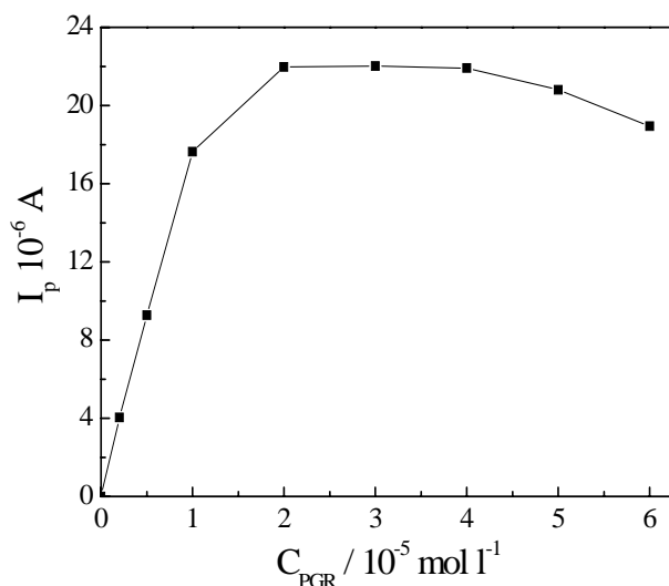
Figure 5. Effect of PGR concentration on the peak current. Other conditions as in Figure 2, curve 3.
