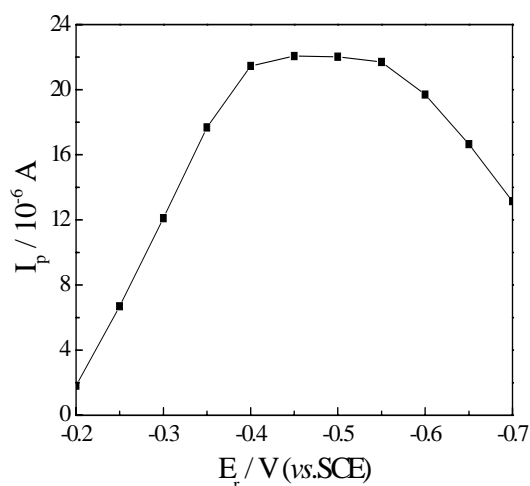
Figure 6. Effect of reduction potential on the peak current. Other conditions as in Figure 2 curve 3.
