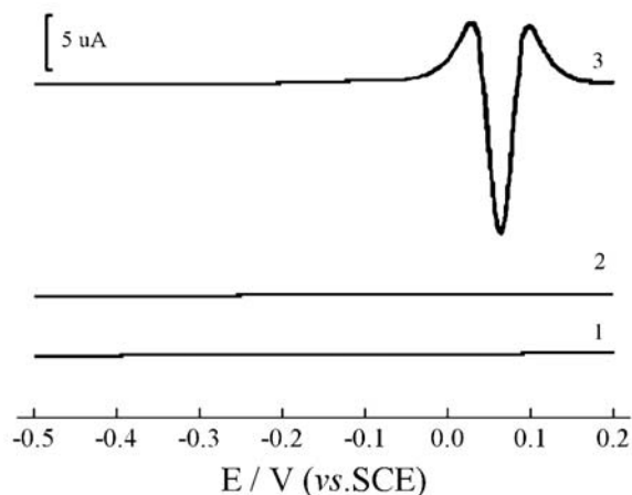
Figure 2. Anodic stripping curves of (1) 1.0 \times 10^{-7} mol/L Sb (III); (2) 3.0 \times 10^{-5} mol/L PGR; (3) 1.0 \times 10^{-7} mol/L Sb (III) + 3.0 \times 10^{-5} mol/L PGR. Preconcentration medium, 0.10 mol/L HCl; preconcentration time: 150 s; reduction and stripping medium, 0.20 mol/L HCl; reduction time and potential: 60 s, -0.50 V; scan rate: 100 mV/s.
