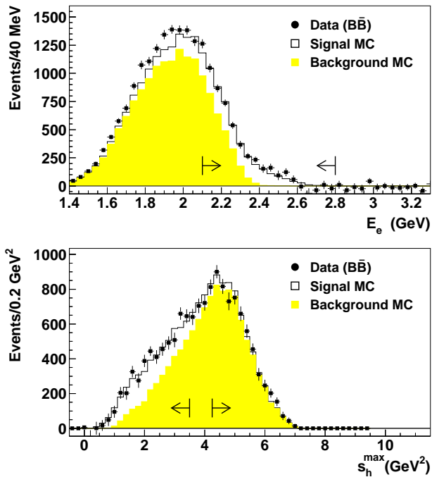
FIG. 2: The electron energy, E_e , and s_h^{\text{max}} spectra in the \Upsilon(4S) frame for continuum-subtracted data and simulated B\bar{B} events satisfying all selection requirements except for the variable shown. The arrows denote the signal (and sideband) region in E_e and s_h^{\text{max}} . Note that \tilde{E}_e \neq E_e (see text).
