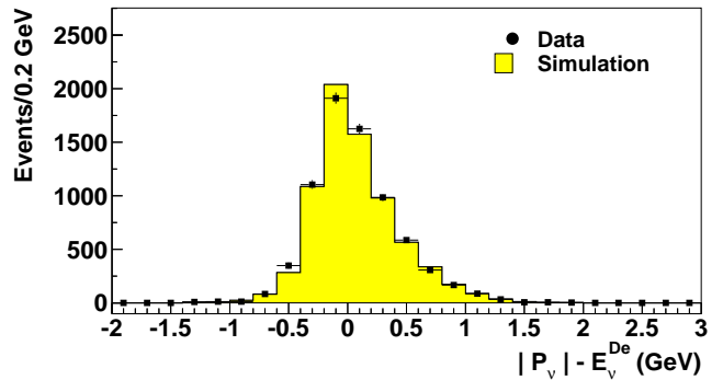
FIG. 1: The difference between the two neutrino energy estimates described in the text for continuum-subtracted data and simulated B\bar{B} events for the De\bar{\nu} control sample.
