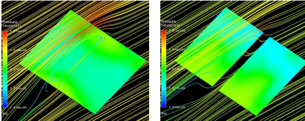
Figure 5: Calculated pressure distribution on the leeward surface of panel without gap (left) and with wide gap (right) at load case 2
