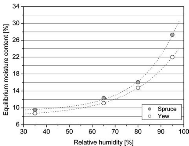
Fig. 2 Sorption isotherms for yew and spruce specimens
