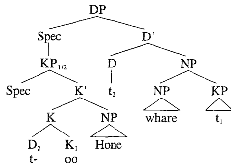
Figure 3. Incorporated possessives.
