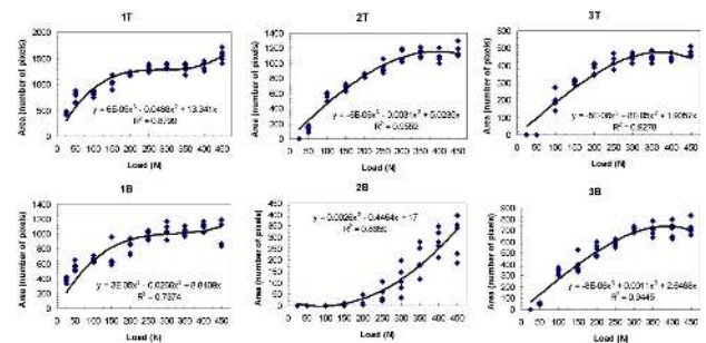
Fig. (6). Mark area vs. specified maximum load curves - upper (T) and lower (B) contacts #s 1-3.
