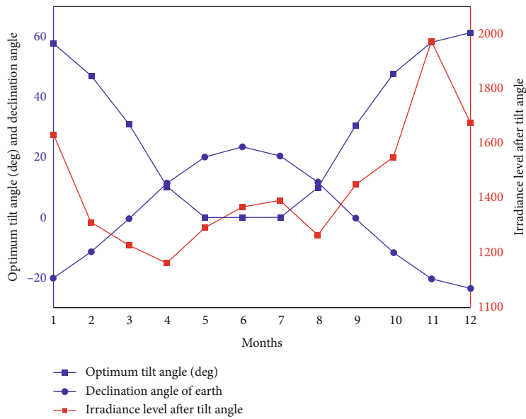
FIGURE 3: Specific monthly irradiance on variable optimal tilt angle and declination angle versus months.
