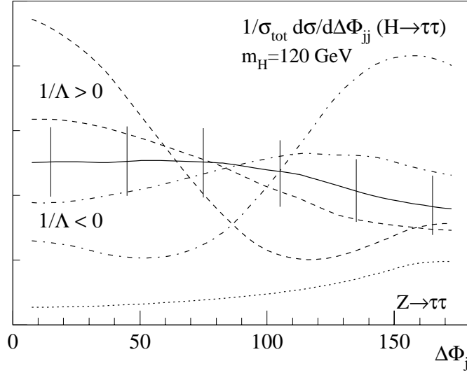
Figure 3. Azimuthal jet angle distribution for the SM and interference with a CP even D5 coupling. The two curves for each sign of the operator correspond to values \sigma/\sigma_{\text{SM}} = 0.04, 1.0 . Error bars for the signal and the dominant backgrounds correspond to an integrated luminosity of 100 \text{ fb}^{-1} per experiment, distributed over 6 bins, and are statistical only.
