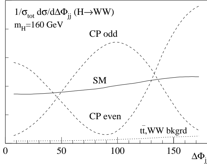
Figure 2. As in Fig. 1, for H \rightarrow WW \rightarrow l\bar{\nu}l\nu at M_H = 160 GeV, with acceptance cuts as in Eq.(4) and Ref. [6]. The dominant backgrounds are t\bar{t} +jets and electroweak WW production.
