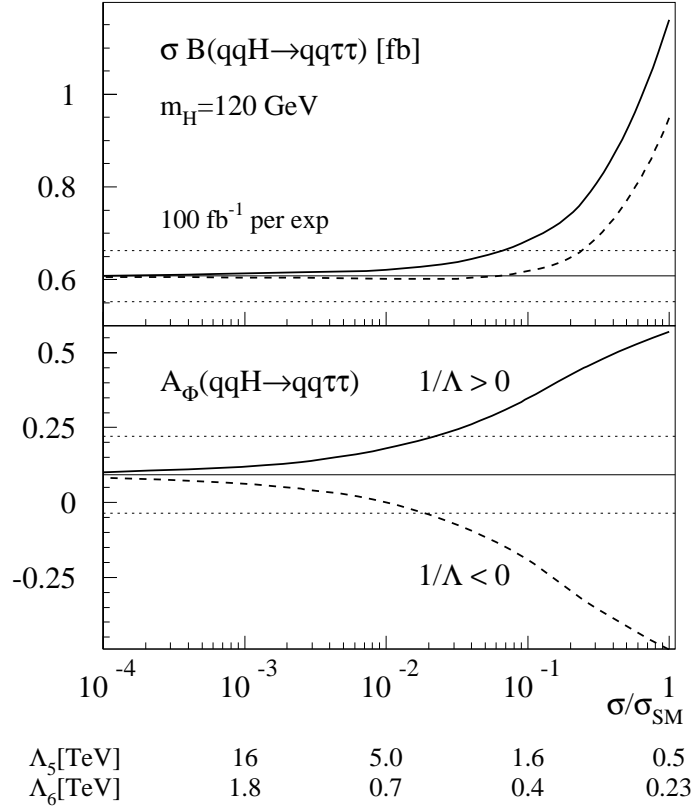
Figure 4. Comparison between a total cross section (counting) experiment and the azimuthal angle asymmetry, Eq.(6), to determine an interference with a CP even D5 coupling. The horizontal lines represent one sigma statistical deviations from the SM value. The secondary axes show the corresponding values of \Lambda_5 and \Lambda_6 , as defined in Eqs.(1,2).
