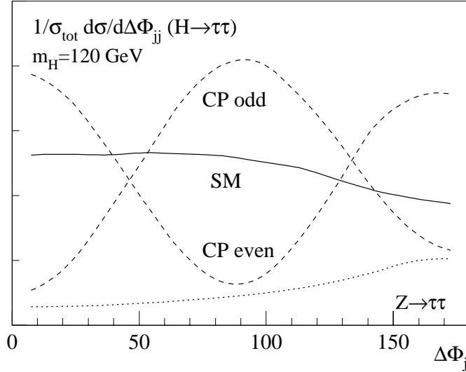
Figure 1. Azimuthal angle distribution between the two tagging jets for the signal and dominant \tau\tau backgrounds, M_H = 120 GeV. Cross sections for the D5 operators are normalized to the SM value, after cuts as in Eq.(4) and Ref. [3]. The expected SM background is added to all three Higgs curves.
