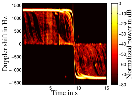
Fig. 7. Calculated Doppler spectra versus scenario time of two oncoming cars.
