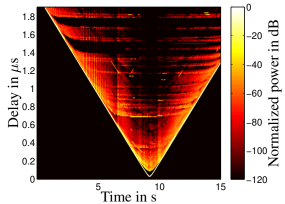
Fig. 8. Power delay profiles of the scenario with oncoming cars.
