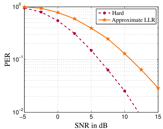
Fig. 11. Performance evaluation of hard and soft (approximate LLR) decision in the VTV-EO scenario.
