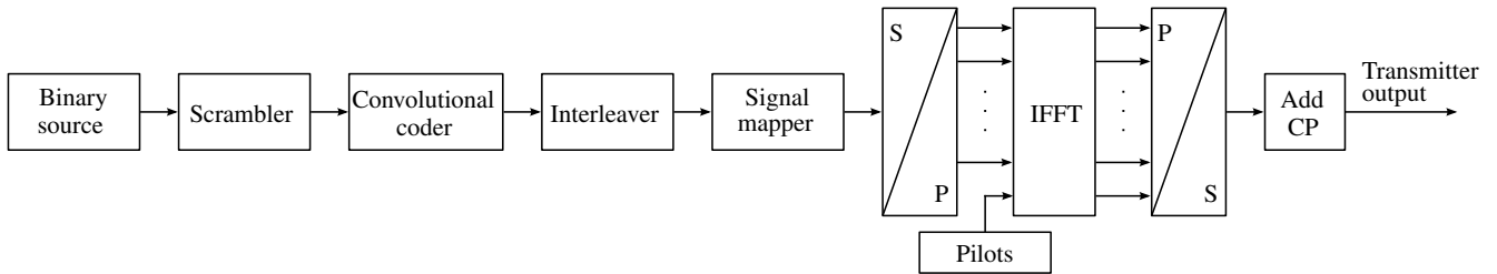
Fig. 3. Block diagram of the transmitter.
