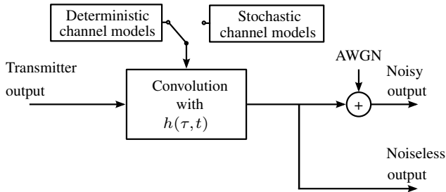
Fig. 4. Block diagram of the radio channel with deterministic and stochastic channel models.
