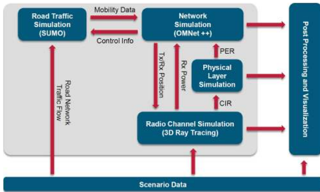
Fig. 1. Integrated simulation environment for C2X communications.
