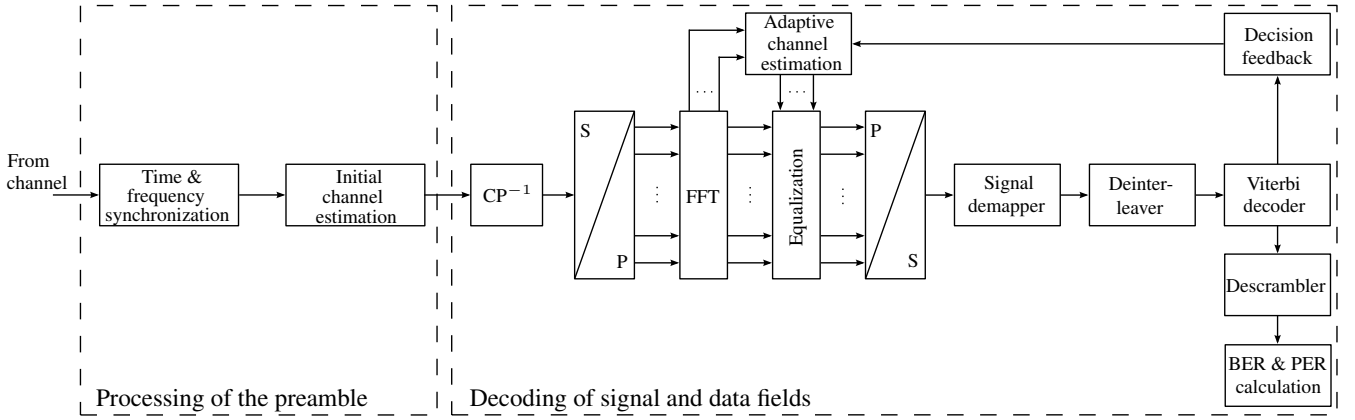
Fig. 5. Block diagram of the receiver.
