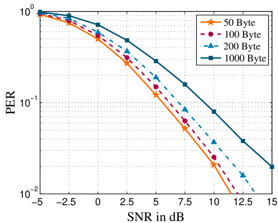
Fig. 10. Impact of the payload size on PER performance in the VTV-EO scenario.
