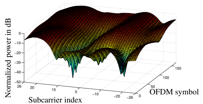
Fig. 9. Realization of a doubly selective channel transfer function of the RTV-SS scenario.
