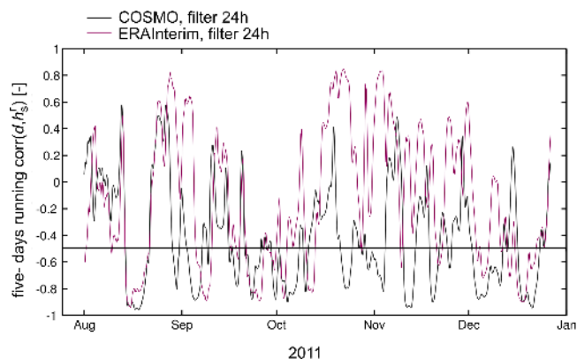
Fig. A1. Comparison of the 5-day moving window correlation between 24 h filtered d and diagnosed source h_s^r with COSMO (grey) and with ERA-Interim (violet). The horizontal black line shows the \text{corr}(d, h_s^r) = -0.5 line used as a threshold for the HRA event definition in Sect. 5.3.
