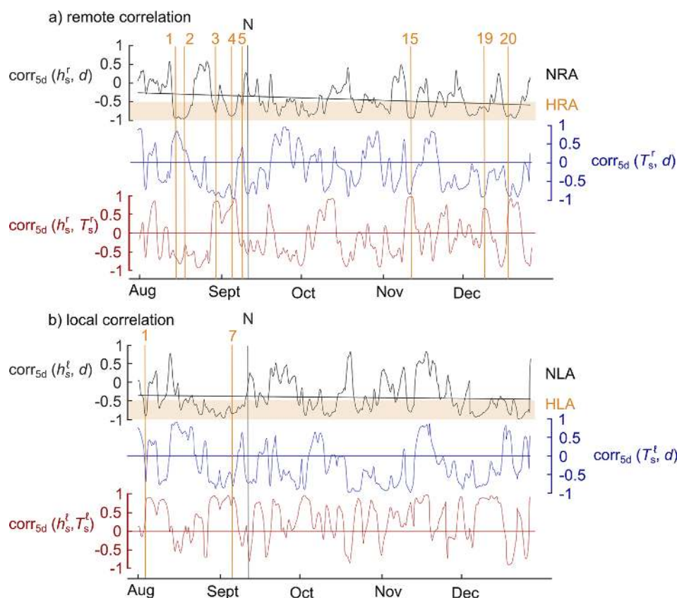
Fig. 8. (a) Five-day moving window correlation between 24 h filtered d measurements and moisture source h_s^r and T_s^r conditions. The orange band in the \text{corr}_{5\text{day}}(h_s^r, d) plot identifies HRA events. Time periods with 0.5 > \text{corr}_{5\text{day}}(h_s^r, d) > -0.5 are identified as NRA events. The black solid line in the \text{corr}_{5\text{day}}(h_s^r, d) plot represents a linear fit to the moving window correlation curve. The straight blue and red lines show \text{corr}_{5\text{day}}(T_s^r, d) = 0 and \text{corr}_{5\text{day}}(h_s^r, T_s^r) = 0 . (b) As in (a) but moving window correlations are shown for local conditions. A few selected HRA and HLA events in (a) and (b) are marked by orange vertical lines (see text for details). The grey vertical line (N) indicates a 5-day period in which we find no anticorrelation of d either with locally measured h_s^l or with remote h_s^r . The dates for the HRA and HLA events are given in Tables 5 and 6, respectively.
