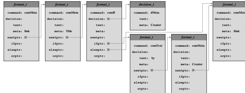
Figure 43 Data structures built for sample format statement
