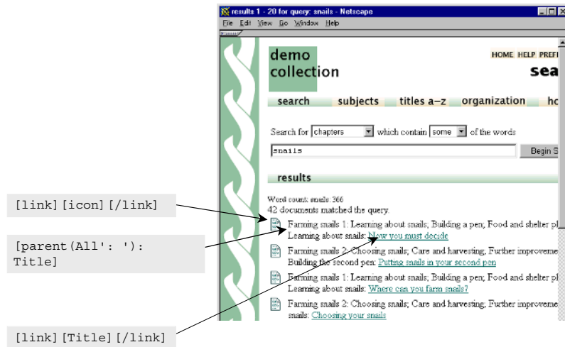
Figure 18 Formatting the search results
