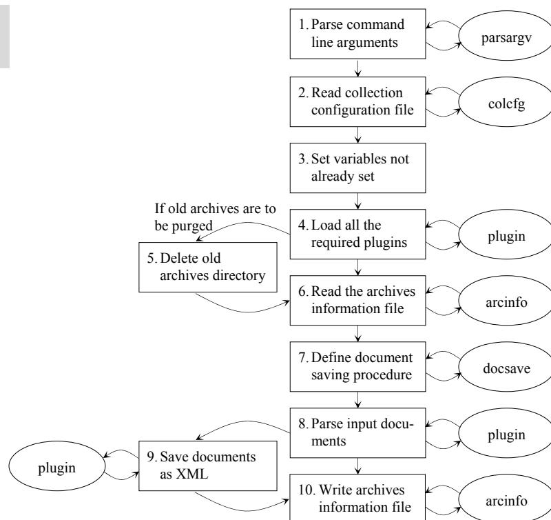
Figure 5 Steps in the import process
