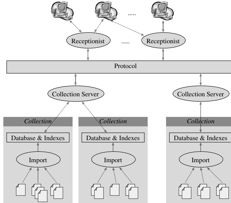
Figure 20 Overview of a general Greenstone system
