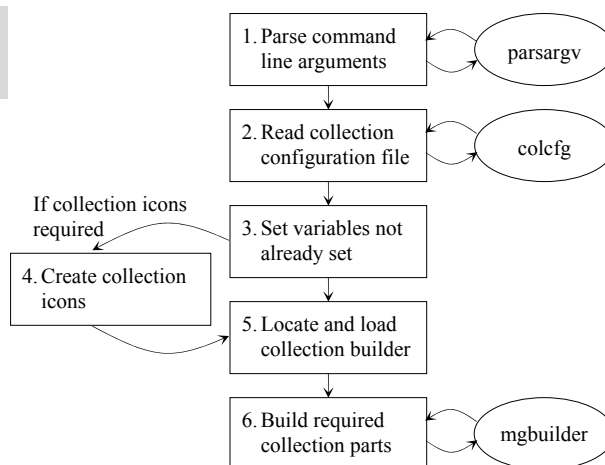
Figure 6 Steps in the build process
