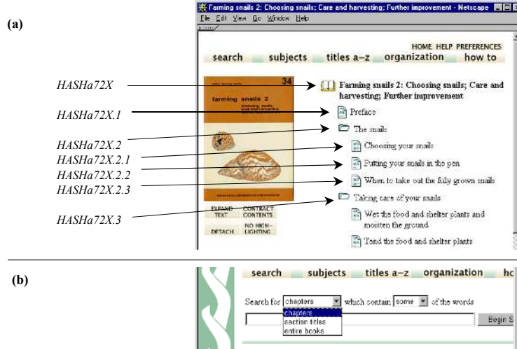
Figure 8 Hierarchical structure in the Demo collection
