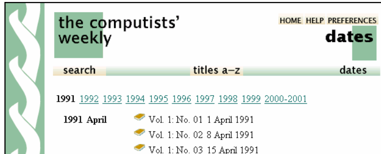
Figure 13 DateList classifier
