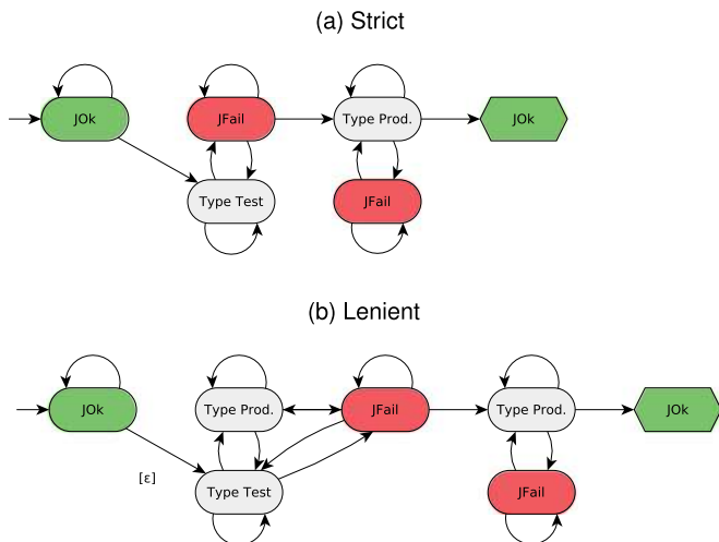
Fig. 7. Strict and lenient NFAs of TDD. JOk stands for a passing and JFail for a failing test execution (JUnitExecution).
