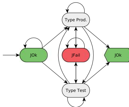
Fig. 8. NFA for the refactoring phase of TDD.
