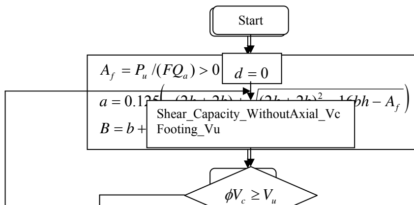
Figure 2.70 Flowchart to compute remaining dimensions, subroutine Footing_Vu
