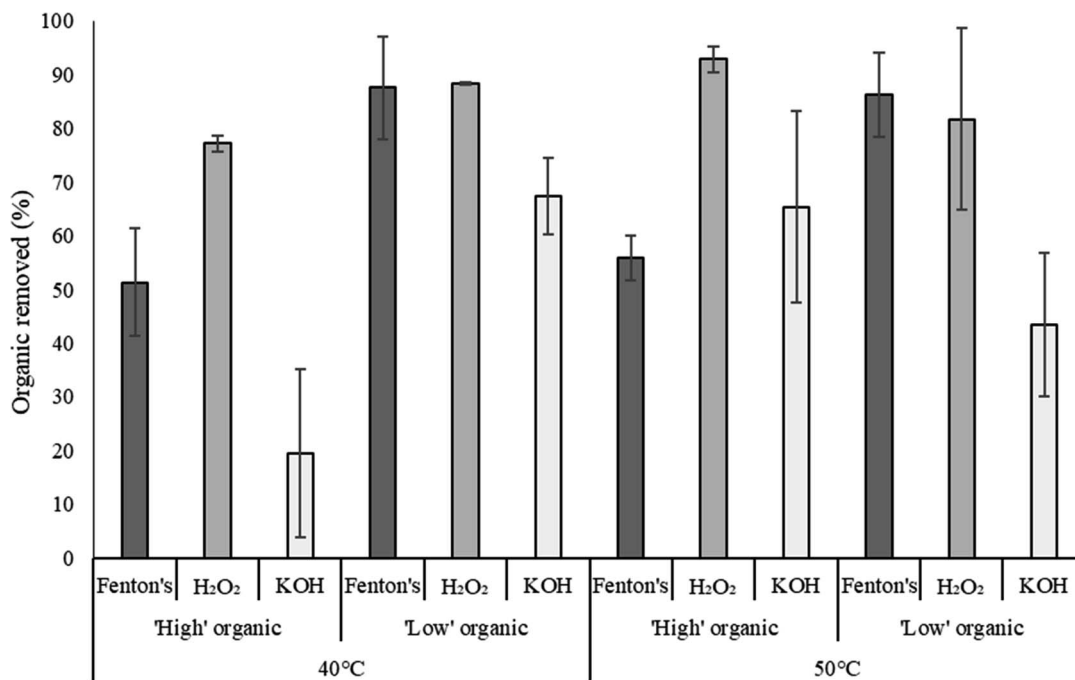
Fig. 1 Organic removed by tested chemicals (Fenton's reagent, potassium hydroxide (KOH)) and hydrogen peroxide ( \text{H}_2\text{O}_2 ) at 40 and 50 °C in samples of initial high ( 73 \pm 0.6\% SE) and low ( 12 \pm 0.9\% SE). Organic matter content. Percent organic removed is reported as a mean ( n = 3 ) with 95% CI error bars.
