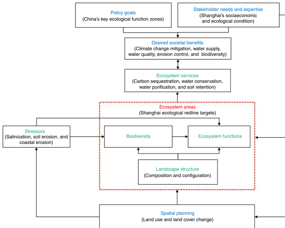
Fig. 1 Science-policy framework linking institutional and ecological information. Ecosystem services provisioning depends on biodiversity and ecosystem functions, which are influenced by landscape structure and stressors (ecological criteria, green text). Spatial planning should manage ecosystem areas (spatial targets, red box/text) to sustain biodiversity and ecosystem functions (ecological health) by minimizing stressors and fragmentation. Ecosystem services assessments for planning should use policy goals and local stakeholder needs to select the desired ecosystem services to ground the analysis in the given decision-making context (socioeconomic criteria, blue text). Black text is the selected ecological and socio-economic criteria to determine the ecological redline areas for Shanghai Municipality. China's Ecological Redline Policy aims to use spatial planning to safeguard ecological redlines areas (ERAs) to ensure the protection of key ecological function zones and ecologically fragile areas (vulnerable to stressors) to improve the living environment for people and biodiversity
