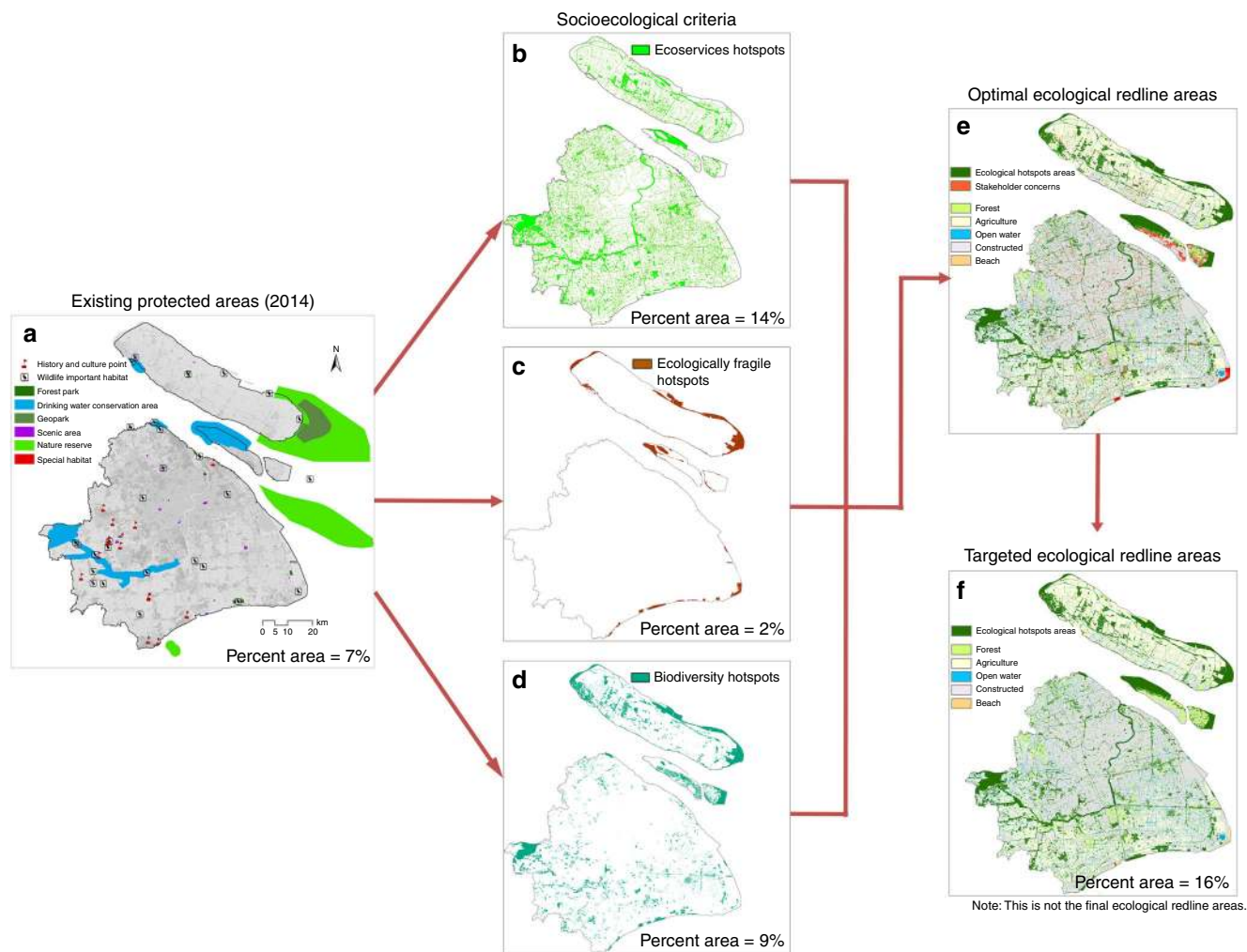
Fig. 3 Spatial results for each step of the spatial planning process to select the ecological redline areas for Shanghai Municipality. a Existing protected areas for 2014, small patches with limited connectivity, representing only 7% of Shanghai's land area. We used the Ministry of Environmental Protection criteria to formulate three indicators for determining optimal ERAs: b ecosystem services hotspots; c ecologically fragile hotspots; and d biodiversity hotspots. Next optimal ERAs (determined from socioecological criteria) were presented to stakeholders who refined ERAs. e Stakeholders indicated areas of concern meaning areas they felt were not manageable (i.e., removal of small patches) or pose serious social and economic burdens to communities (i.e., removal of major disagreement areas). f Targeted ERAs are not the final ERAs but Shanghai Municipality is considering using them to form the final ERAs. The maps in this figure were made by the author in ArcGIS software for use in this paper
