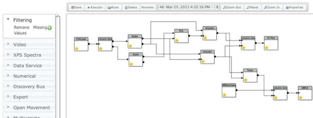
Figure 2. The e-Science Central workflow editor showing one of the chemical modelling workflows. (Online version in colour.)
