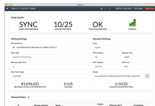
Figure 5. Parity UI Dashboard
