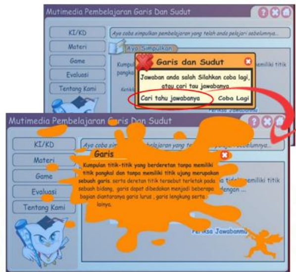
Figure 7. Conclusion page
