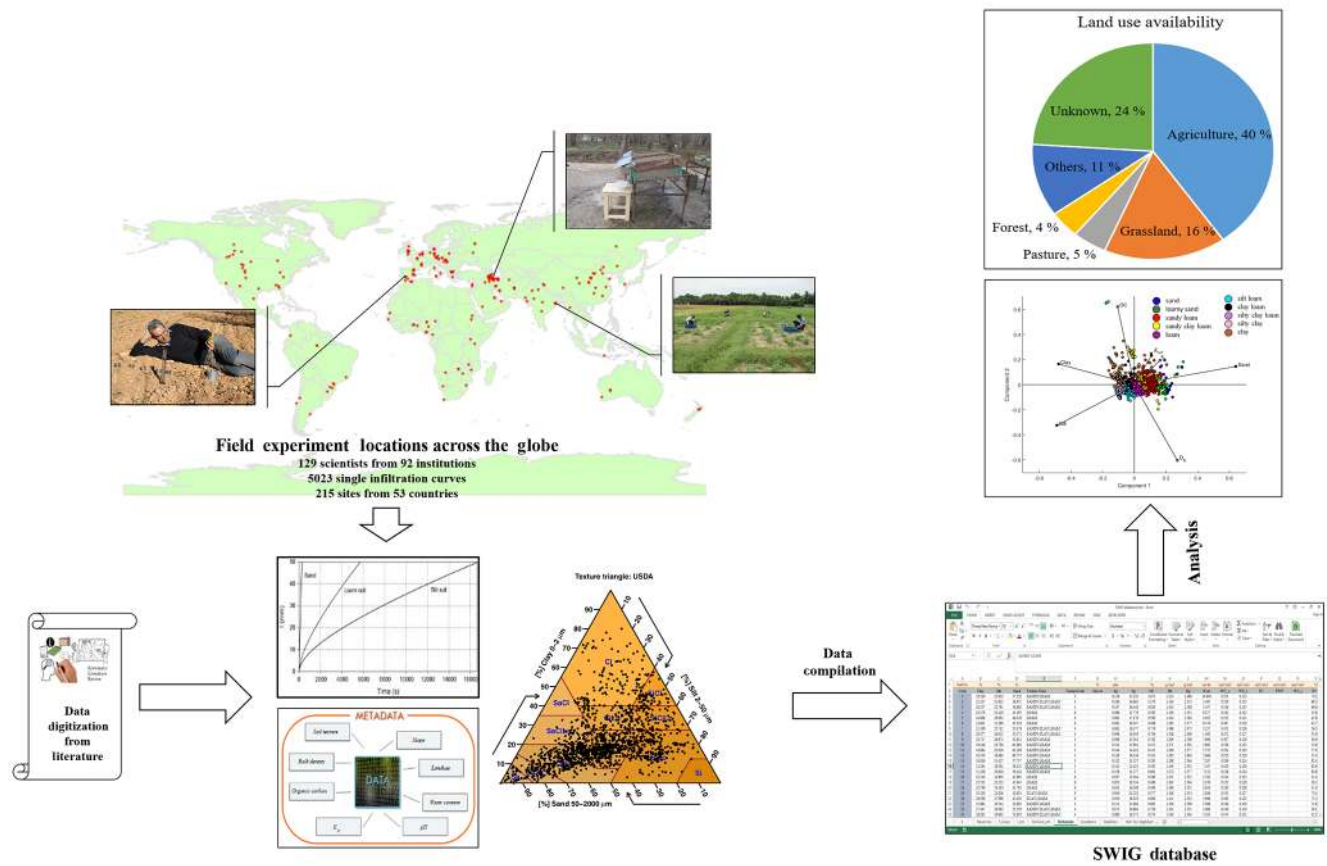
Figure 1. SWIG flowchart.
