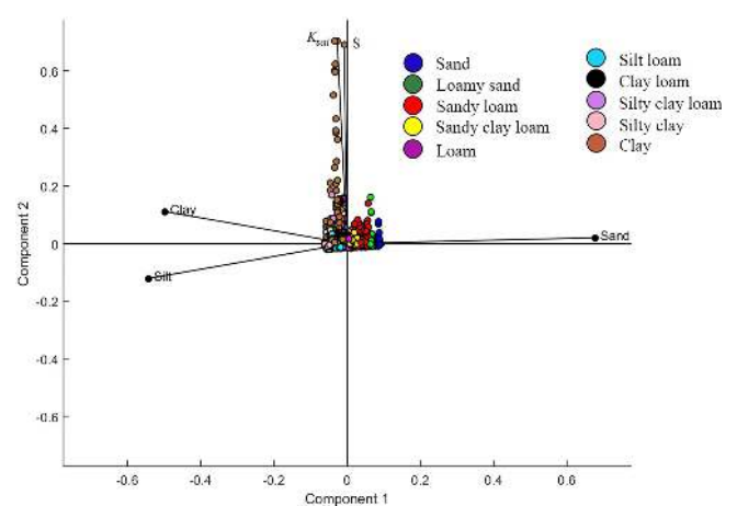
Figure 7. The relationships between clay, silt, sand contents and estimated hydraulic parameters ( S and K_{\text{sat}} ).
