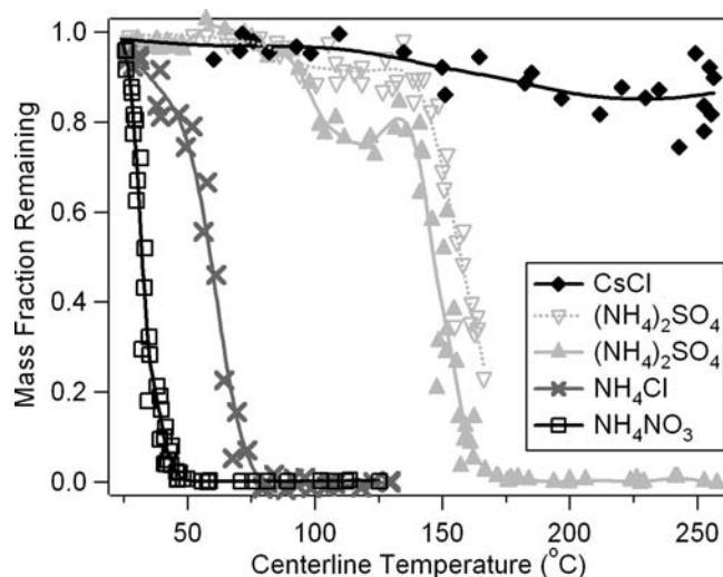
FIG. 6. Response to heating shown as a function of temperature for polydisperse species generated in the laboratory. (NH 4 ) 2 SO 4 curves highlight variability while using the AMS as a particle detector. Lines are spline fits to guide the eye.
