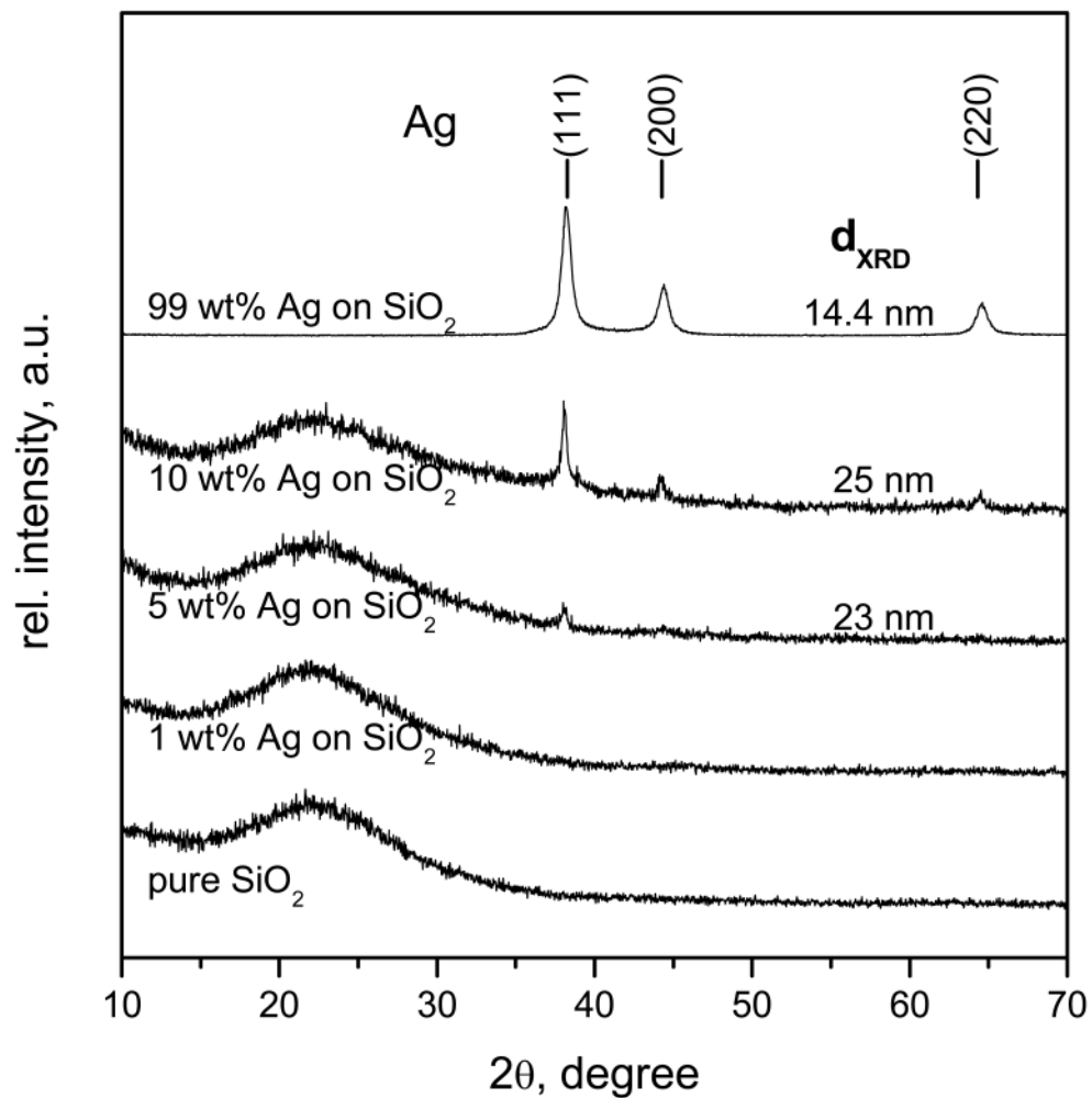
Figure 8. XRD of Ag deposited on the surface of \text{SiO}_2 nanoparticles for different % wt of Ag. The d_{\text{XRD}} size of silver is indicated that comes mostly from the large mode of bimodal Ag size distribution arising from FSP of Ag nitrate solutions (Heine and Pratsinis, 2007). In parenthesis the Miller indices (hkl) of the crystal planes according to the ICSD 64997 is indicated.
