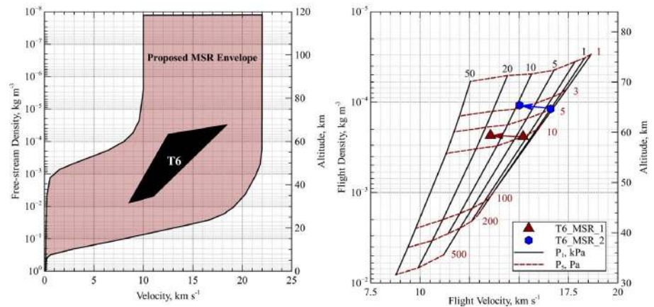
(a) Possible MSR trajectory envelope (adapted from Johnston and Brandis (2015)) with T6 performance prediction.
