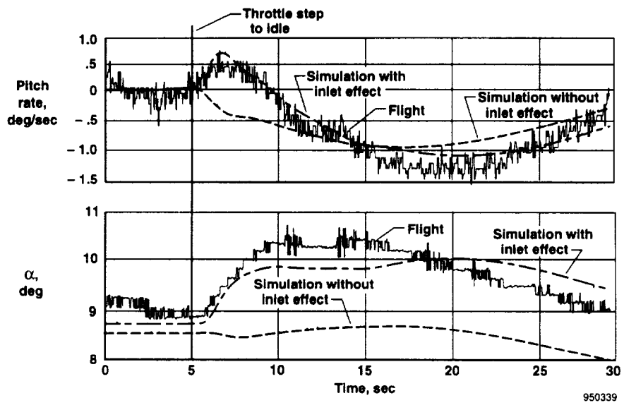
Figure 27. Comparison of flight and simulation for throttle step to idle, with and without inlet-airflow effect, KCAS = 170 knots, flaps up.
