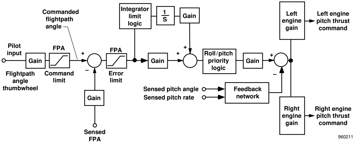
(b) Longitudinal control system. Figure 7. Concluded.
