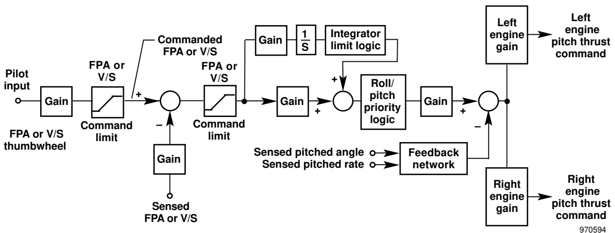
(b) PCA longitudinal control system, center engine modes not shown.
