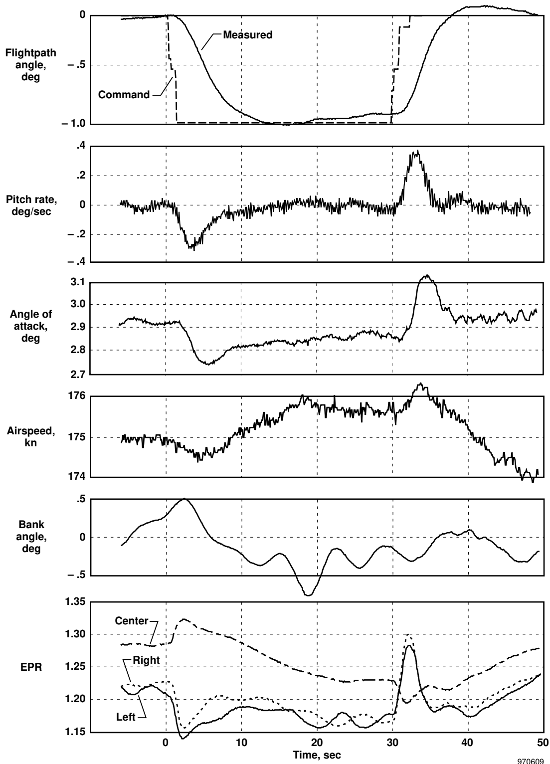
Figure 27. Time history of MD-11 flightpath steps, three-engine dynamic longitudinal mode, 17,000 ft, gear down, Flaps 28.
