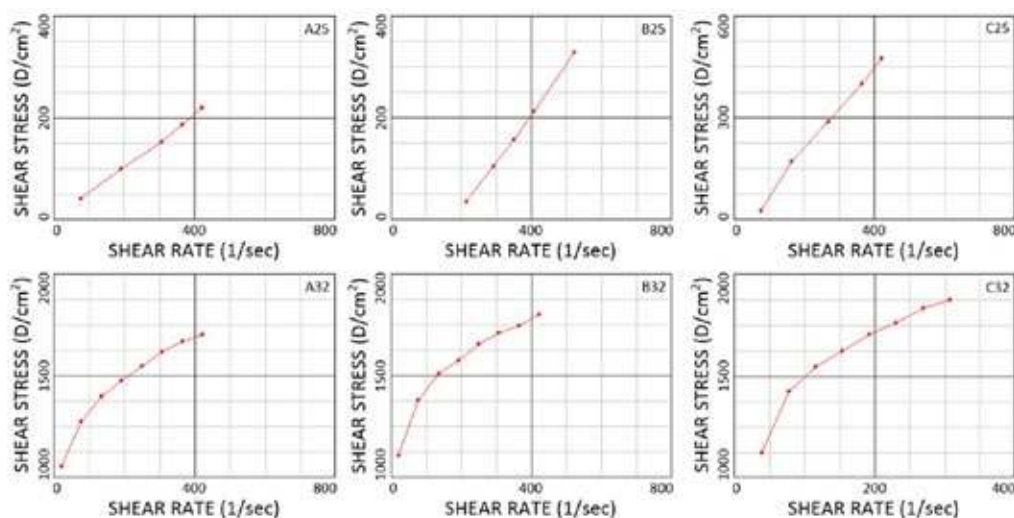
FIGURE 4 - Effect of temperature on rheological behavior of formulations. (A25 F16, 25 °C; B25 P16, 25 °C; C25 FH1405, 25 °C; A32 F16, 32 °C; B32 P16, 32 °C; C32 FH1405, 32 °C).
