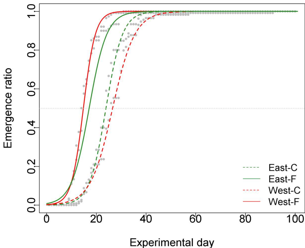
Figure 5.1 Predicted cumulative emergence ratio over time (experimental day) across temperature treatments (Current Temperature, C and Future Temperature, F) and region (East and West) using a binomial error distribution. Grey dots represent observed data.
