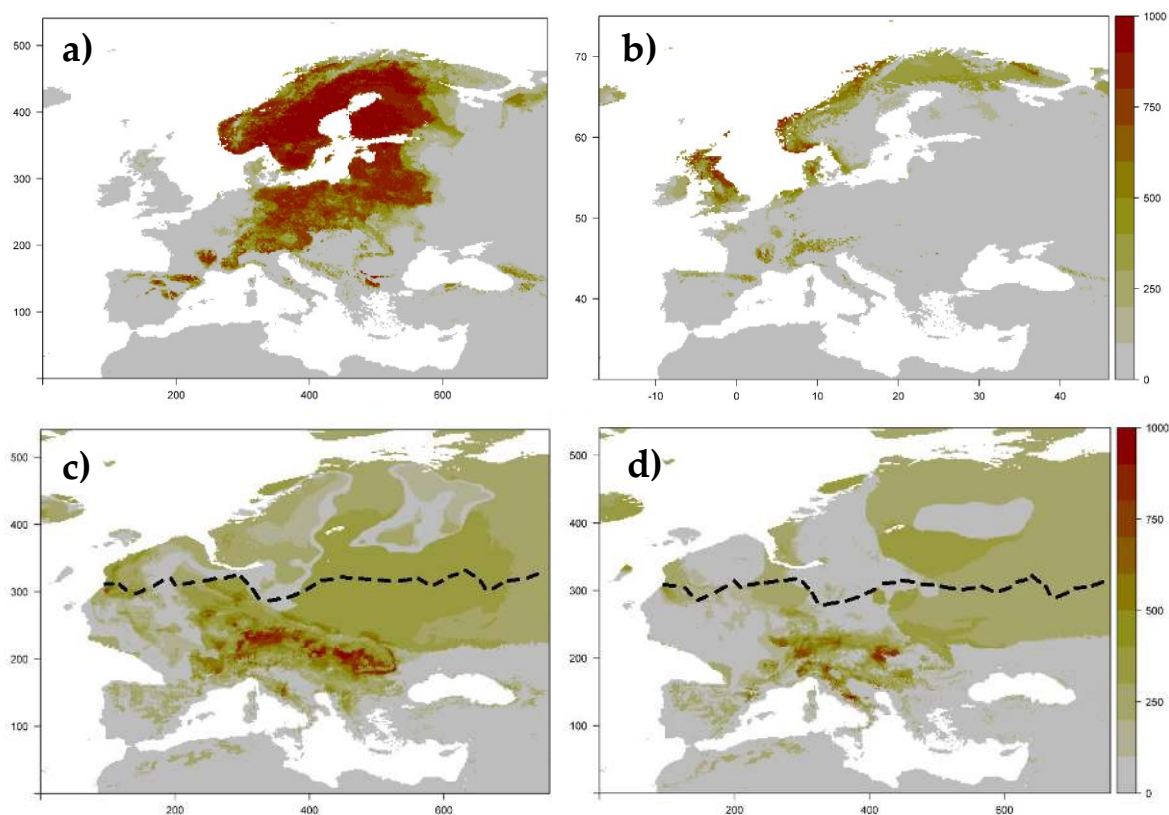
Figure 2.7 Projection of species under (a) current climatic conditions; (b) past climatic conditions in the Last Interglacial Period (i.e. LIG); (c) past condition in the last glacial maximum using CCSM global circulation model (i.e. LGC-CCSM), and (d) past condition in the last glacial maximum using MIROC global circulation model (i.e. LGC-MIROC). The black line shows approximately where the ice sheet limit was during the last glacial maximum.
