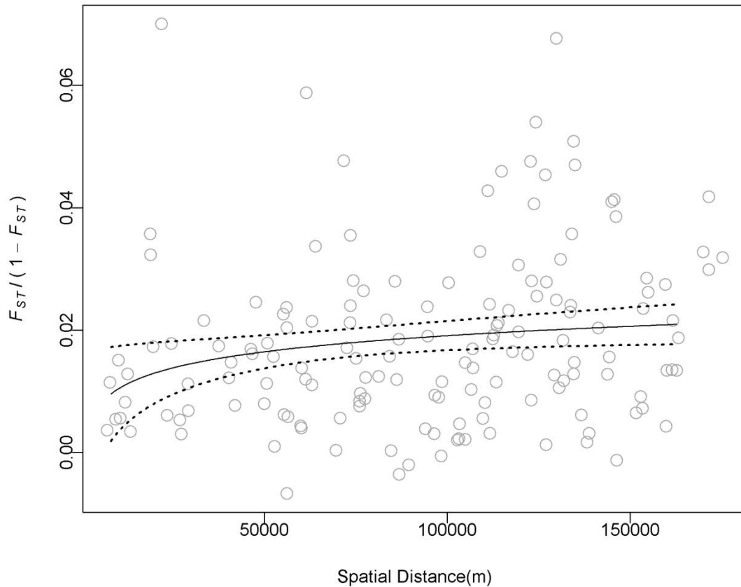
Figure 3.3 - Isolation by distance. Black line represent the slope of the correlation of the spatial distance (m) against F_{ST}/(1-F_{ST}) after 10,000 permutations of sites among locations.
