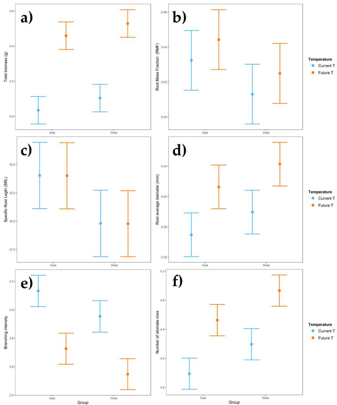
Figure 5.2 Model predictions for (a) total dry biomass, (b) root mass fraction RMF, (c) Specific Root Length SRL, (d) root average diameter, (e) branching intensity and (f) number of stomata rows of Scots pine seedlings from the two regions (East vs. West) across the temperature treatment (Current T, Future T). Error bars represent \pm SE.
