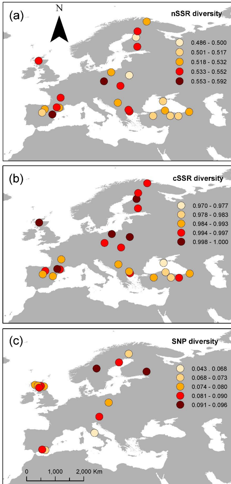
Figure 2.5 Diversity estimated using different markers: (a) nuclear (nSSR diversity), (b) chloroplast (cSSR diversity), and (c) SNP (SNP diversity) for European populations of Scots pine .
