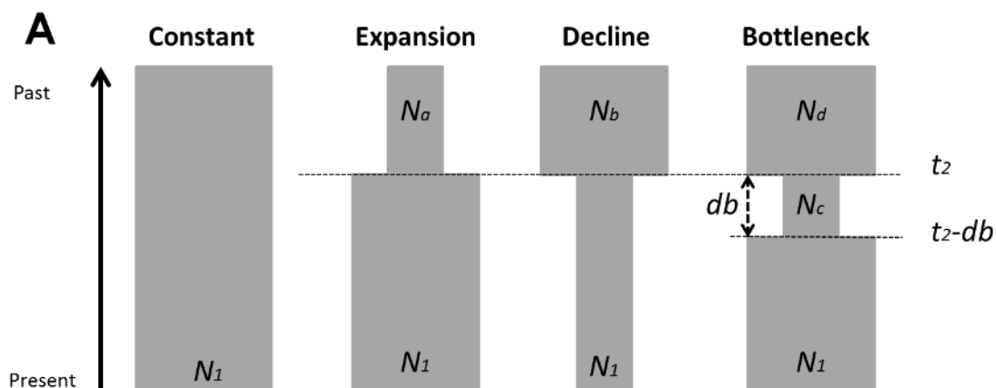
Figure 2.4 Scenarios of changes in population size of Scots pine tested, that assume (i) constant (i.e. no change in population size), (ii) expansion, (iii) decline, or (iv) bottleneck. Parameters N_1 , N_a , N_b , N_c and N_d refers to effective population sizes, t_2 is the time in generations at which the change in population size occurred and db is the duration of the bottleneck.
