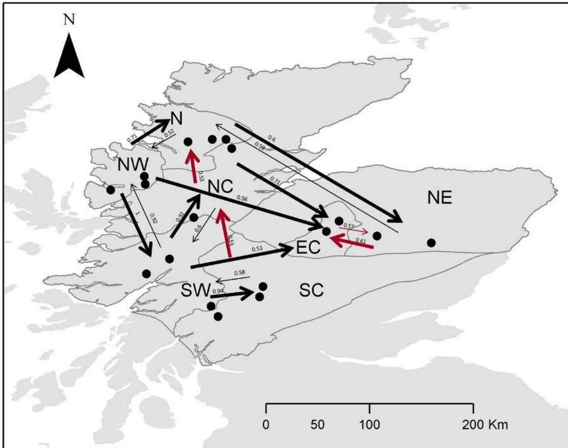
Figure 3.4 - Relative migration networks for nSSR with populations sorted in seed groups which are defined by grey lines and letters (see Table 3.2 for population and seed group details) using a threshold of 0.5. Arrows in black denote greater gene flow pattern in the W-E direction, whereas arrows in red denote greater gene flow in the E-W or S-N direction. Thicker arrows mean stronger gene flow in such direction.
