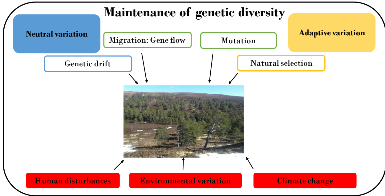
Figure 1.1 Processes and forces (in red) influencing neutral and adaptive genetic variation.
