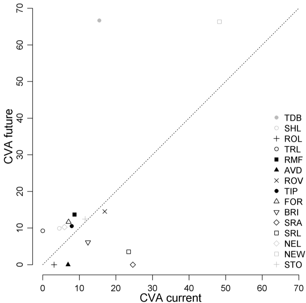
Figure 5.3 Plasticity to change of the coefficient of genetic variation ( C_{VA} ) of Scots pine seedlings across the temperature treatment (current and future). Refer to table 5.4 for trait code key. Grey symbols represent above ground traits, whereas black symbols represent below ground traits. Symbols above the dashed 1:1 line indicate higher C_{VA} under future conditions.
