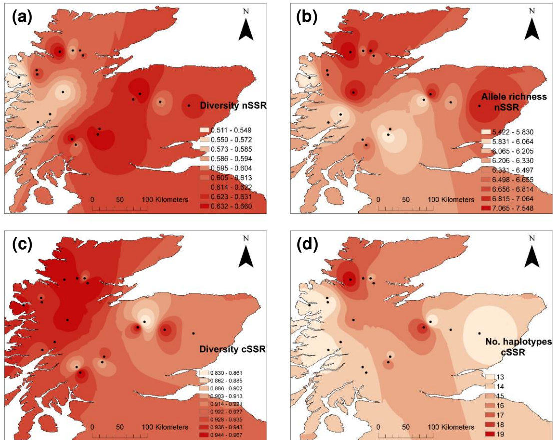
Figure 3.2 - Genetic diversity parameters for nSSR (above) and cSSR (below). (a) Genetic diversity for nSSR ( nH_E ); (b) Rarefied allele richness for nSSR ( nA_R ), (c) Gene diversity corrected for sample size for cSSR ( cH_E ); (d) no. of haplotypes for cSSR ( cH_N ).
