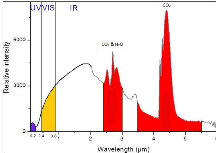
Figure 2: Typical emission spectrum of hydrocarbon fire
