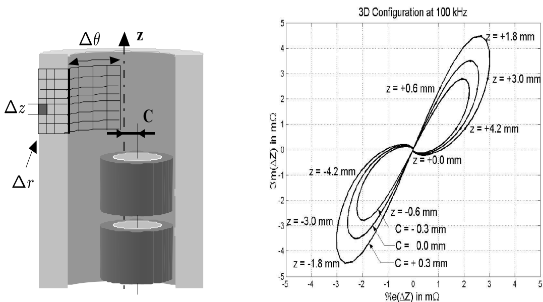
FIGURE 8. Transversal flaw: impedance plane diagram for a non centered probe operating at 100 kHz in differential mode for three values of eccentricity: C = -0.3 , C = 0 mm and C = +0.3 mm.
