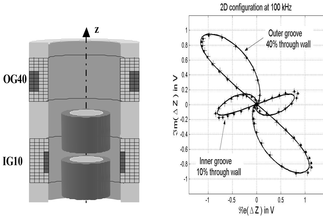
FIGURE 2. Circumferential OG40 and IG10 flaws: schematic and EC signal plane diagram for a centered probe operating at 100 kHz in differential mode ('—' experimental data, '•' 2D model, '+' 3D model).
