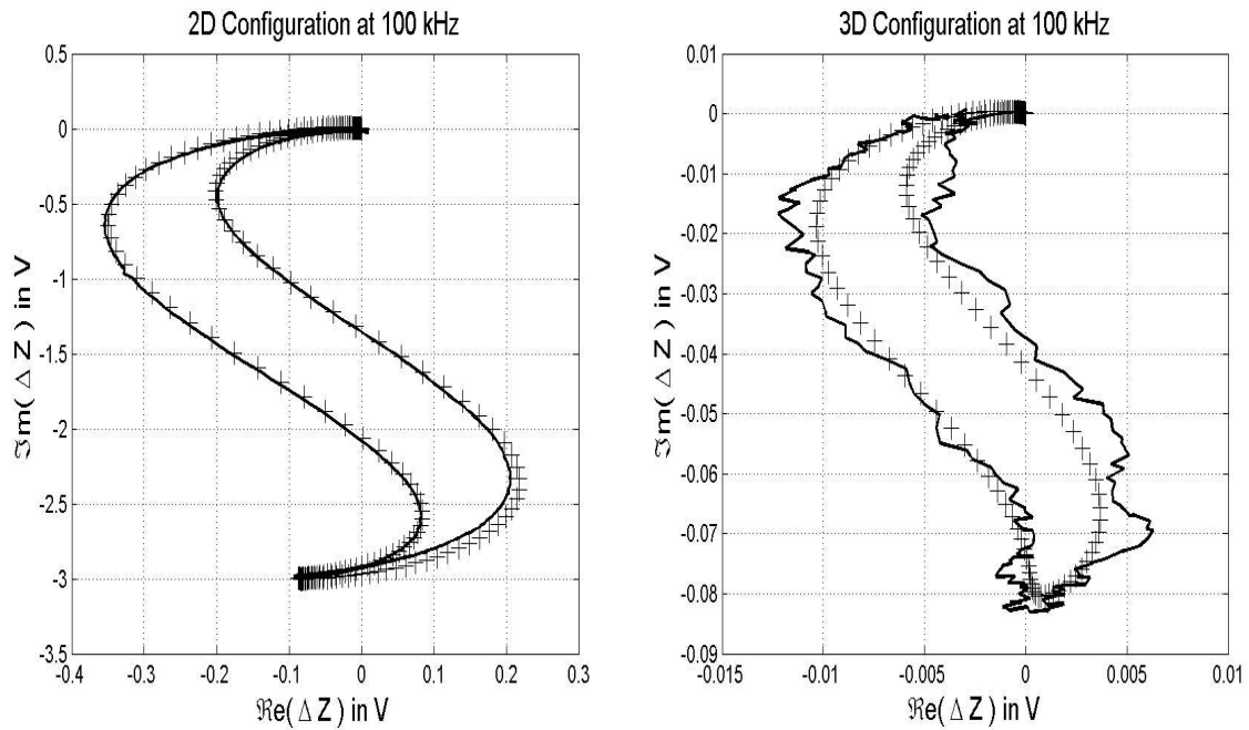
FIGURE 6. Circumferential OLG30 (left) and longitudinal LN54 (right) flaw: EC signal plane diagram for a centered probe operating at 100 kHz in pseudo absolute mode ('-' experimental data, '+' 3D model).
