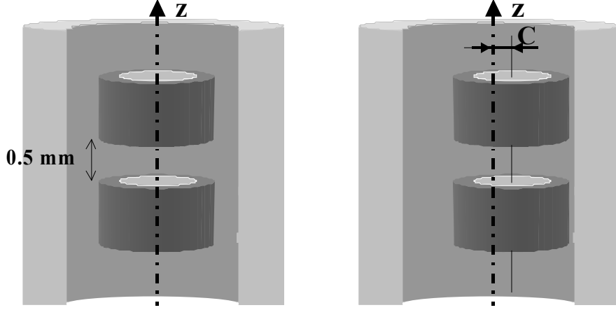
FIGURE 1. Schematic of the two bobbin coils probe used to inspect a conducting tube. The tube, made of inconel 600 (conductivity of 1 MS/m), has an inner radius of 9.84 mm and a thickness of 1.27 mm. The probe consists of two identical coils excited with a time harmonic drive current in phase in both coils (additive flux mode). The inner radius of the coils is 7.83 mm, the outer radius is 8.5 mm, the height is 2 mm, the number of turns is 70, the gap between the coils is 0.5 mm. The probe may moves straight along the tube axis (at left) or it may be non centered on the tube axis considering an eccentricity C (at right).
