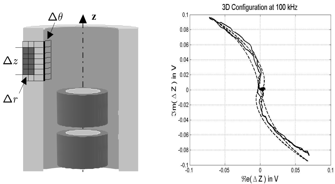
FIGURE 4. Longitudinal LN54 notch: schematic and EC signal plane diagram for a centered probe operating at 100 kHz in differential mode ('-' experimental data, '-' 3D model).
