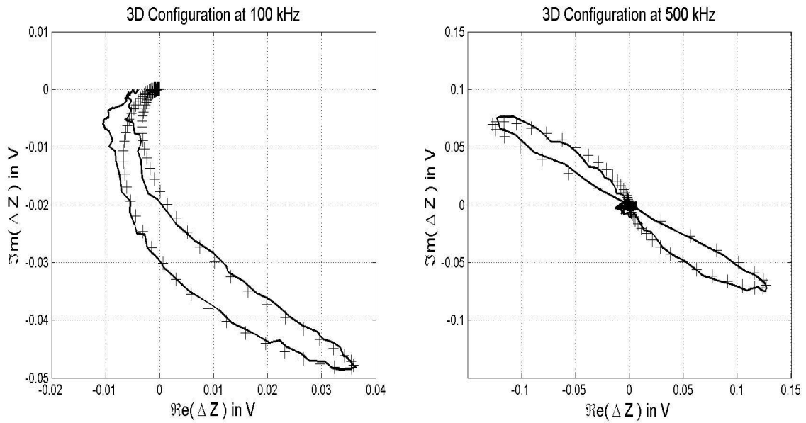
FIGURE 7. Transversal TN100 flaw: EC signal plane diagram for a centered probe operating in pseudo absolute mode (left) at 100 kHz and in differential mode (right) at 500 kHz (‘-’ experimental data, ‘+’ 3D model).
