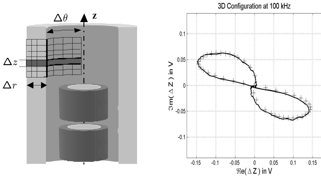
FIGURE 3. Transversal TN100 notch: schematic and EC signal plane diagram for a centered probe operating at 100 kHz in differential mode ('-' experimental data, '+' 3D model).
