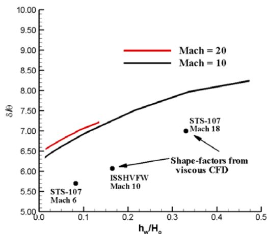
Figure 5. h_w/H_0 vs. \delta/\theta at X/l = 0.3 along Orbiter centerline at \alpha = 40 degrees for equilibrium air flow.
