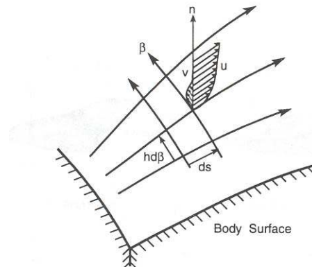
Figure 3. Typical surface streamline and boundary layer profile
