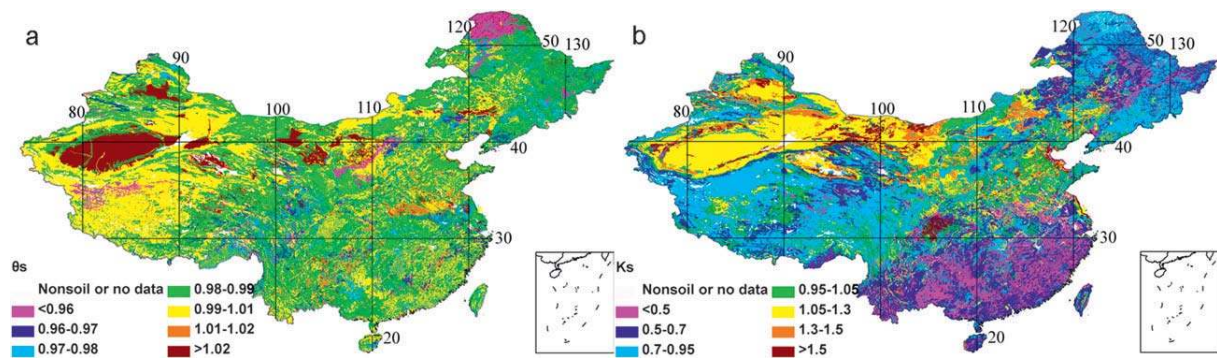
FIG. 5. The difference of saturated water content ( \theta_s , \text{cm}^3 \text{cm}^{-3} ) and saturated hydraulic conductivity ( K_s , \text{cm day}^{-1} ) of layer 2 (0.045–0.091 m) estimated by PTFs of FCH and FGM (FCH divided by FGM).
