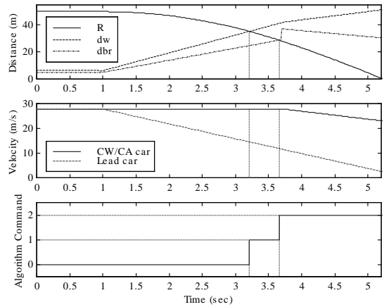
Figure 8: Honda's Algorithm in Degraded Conditions
