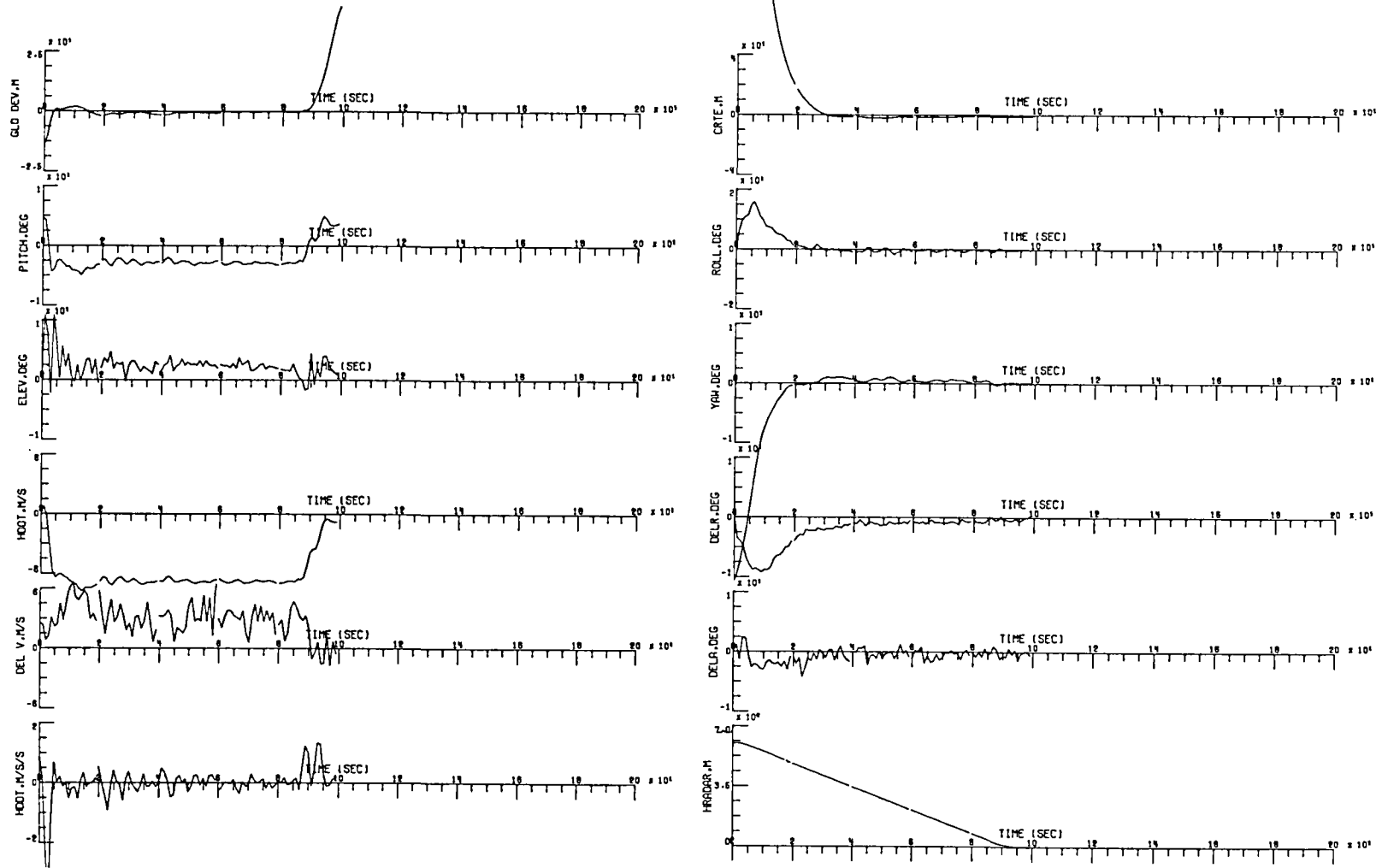
Figure 19 Final Approach Simulation: 64.3 m/sec (125 knot) airspeed
