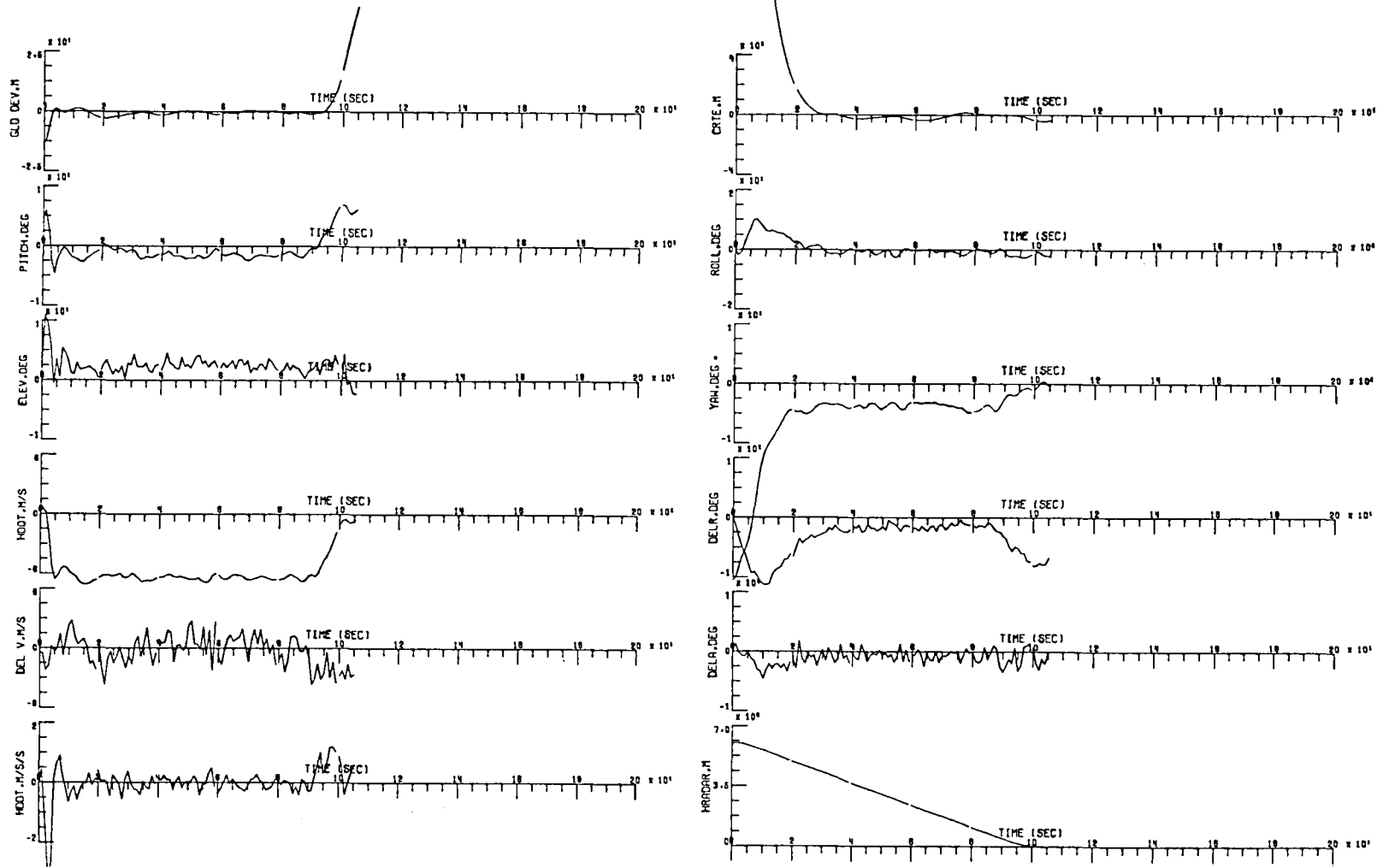
Figure 13 Final Approach Simulation: cross-wind, average turbulence
