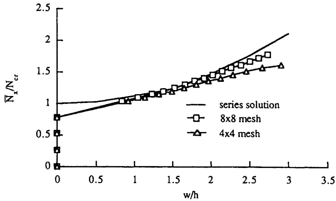
Figure 4 Comparison of postbuckling responses of Gl/Ep single layered orthotropic plate; N_{cr} = 1.918 \times 10^5 lb/in.
