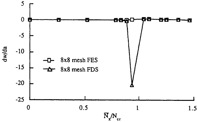
Figure 11 Comparison of sensitivities of central deflection ( dw/da ); GI/Ep single layered orthotropic plate; complete loading; N_{cr} = 1.918 \times 10^5 lb/in.
