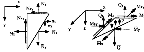
Figure 1 Force analysis of a plate.
