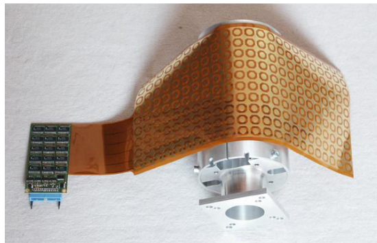
Fig. 7 Cover of forearm with flexible sensor
