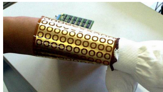
Fig. 3 Flexible sensor array
