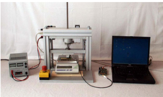
Fig. 9 Testbed
