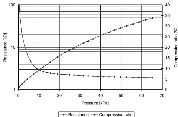
Fig. 10 Characteristics of the cover material
