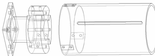
Fig. 6 Cover design
