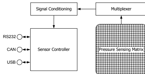
Fig. 1 Sensor system architecture
