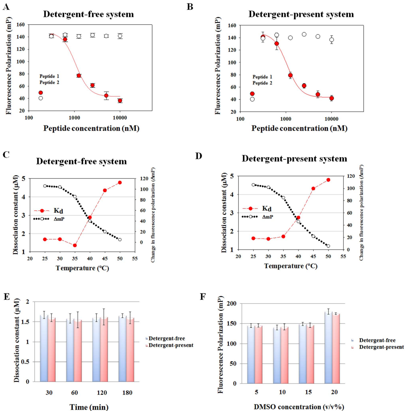
Figure 2. Assay development and stability assessment. A. Unlabeled peptide 1 (Ac-PFKPP-NH 2 ) and mutant peptide 2 (Ac-PAKPP-NH 2 ) were titrated into a mixture of c-Cbl (RING) protein (3 \mu mol/L)+100 nmol/L probe 1 separately in the detergent-free system. IC 50 (peptide 1)=1.05 \pm 0.09 \mu mol/L. B. Unlabeled peptide 1 and mutant peptide 2 were titrated into a mixture of c-Cbl (RING) protein (3 \mu mol/L)+100 nmol/L probe 1 separately in the detergent-present system. IC 50 (peptide 1)=1.06 \pm 0.09 \mu mol/L. C and D, temperature dependence of K_d and \Delta mP values in detergent-free or detergent-present system. c-Cbl (RING) protein was titrated against 100 nmol/L probe 1. E. Assessment of stability of binding experiments over time in detergent-free or detergent-present system. c-Cbl (RING) protein was titrated against 100 nmol/L probe 1. F. Stability of binding experiments with increasing DMSO concentrations in detergent-free or detergent-present system. DMSO was titrated into constant amounts of c-Cbl (RING) protein (3 \mu mol/L) and probe 1 (100 nmol/L) mixture. The total reaction volume was maintained constant in all wells at 20 \mu l. The measurements were made at room temperature (25 ^{\circ}C ) after 30 min of incubation. doi:10.1371/journal.pone.0078042.g002
